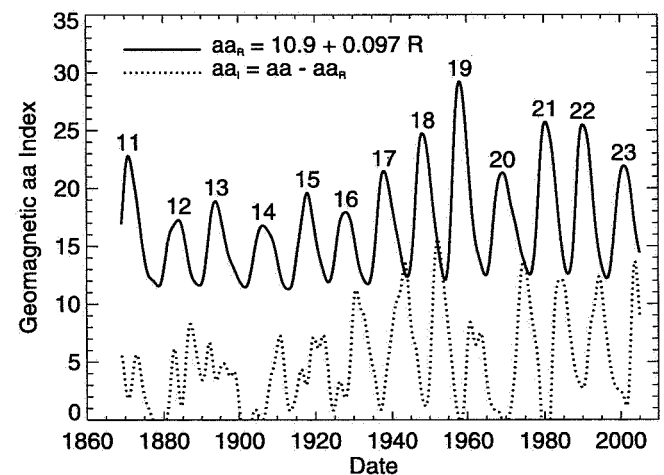
Figure 2. Solar cycle, aa_R , and interplanetary, aa_I , components of geomagnetic activity as functions of time. The solar cycle component is directly proportional to the sunspot number and illustrates the sequence of cycle amplitudes for the last 13 solar cycles (numbered). The interplanetary component has a similar sequence of peaks but they occur several years earlier – usually before the time of cycle minimum.
