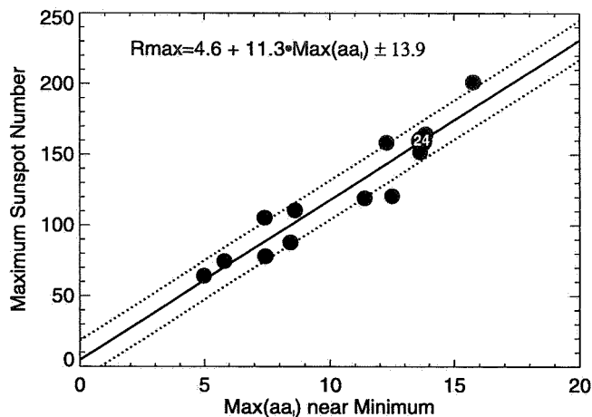
Figure 3. Maximum sunspot number for the following cycle as a function of the maximum in the interplanetary component of the aa index. The following cycle amplitude is well correlated with the earlier peak in aa_1 with little scatter about a linear relationship (solid line with 1-sigma limits shown with dotted lines). The prediction for sunspot cycle 24 is shown with the circled number 24 – a maximum sunspot number of 160 \pm 25 .
