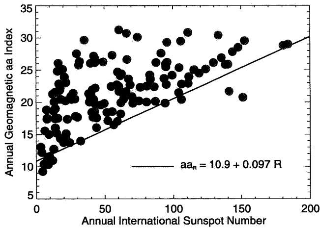
Figure 1. Annual values for the geomagnetic index aa as a function of the corresponding annual International Sunspot Number for the years 1868 to 2005. Both monthly activity indices are smoothed with a 24-month FWHM Gaussian and then sampled at yearly intervals. At a given sunspot number there is a baseline level of geomagnetic activity which is proportional to the sunspot number. Geomagnetic activity extends above this level – particularly late in each solar cycle. This baseline level, aa_R , is determined by fitting a line through the lower boundary of activity.
