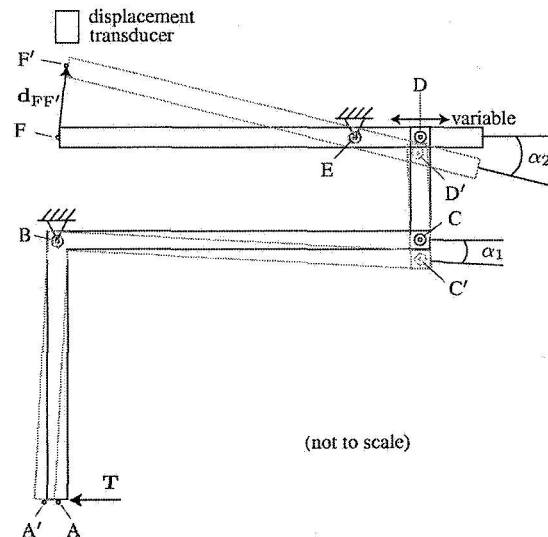
FIG. 2: Schematic illustration of the balance mechanism components in their undeflected and deflected positions (deflected beam positions shown in grey).
