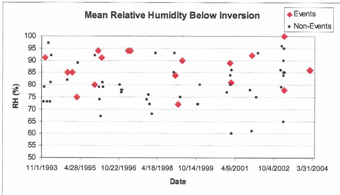
Figure 18. Scatter plot of the mean relative humidity (in %) below the inversion during event (large diamond) and non-event days (small circle).
