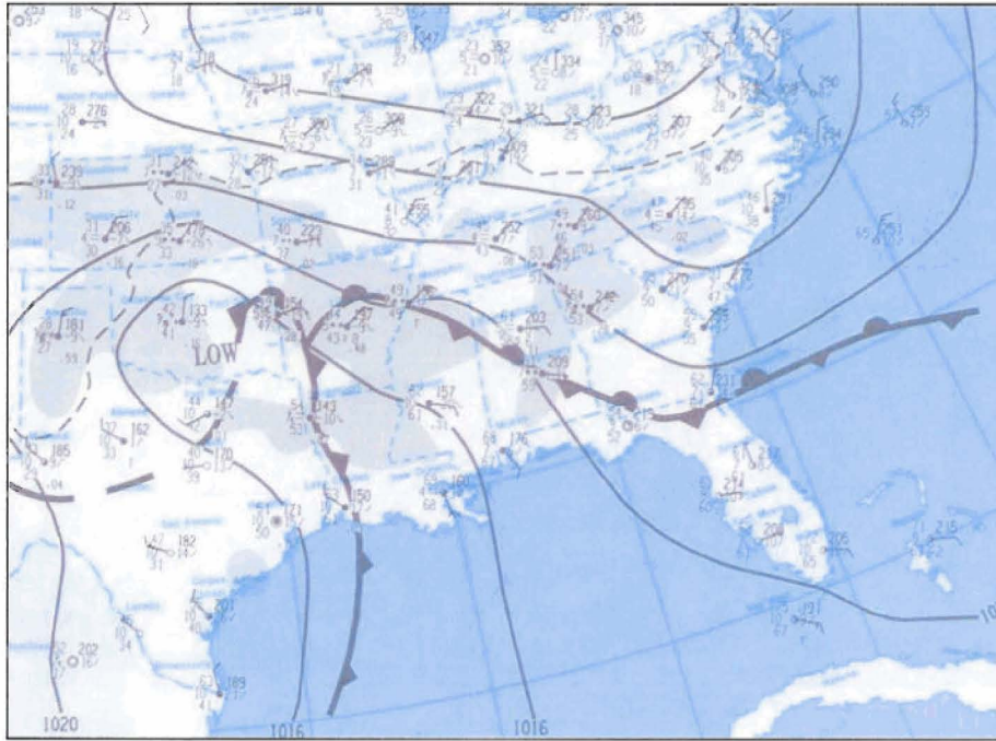
Figure 10. Surface analysis at 1200 UTC on 30 January 1999.
