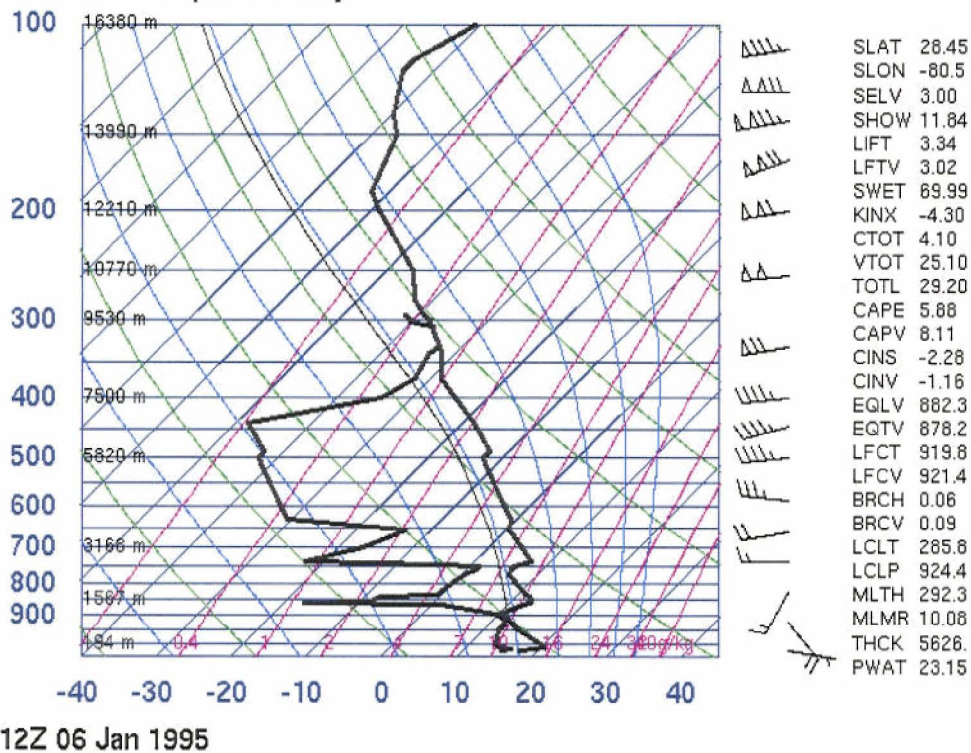
Figure 3. XMR rawinsonde at 1200 UTC 6 January 1995. Note the strong inversion near 900 mb, veering winds with height, and the high relative humidity beneath the inversion.
