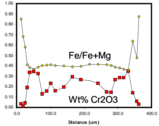
Fig. 3. Microprobe profiles across MIL pyroxene in Fig. 3. Note that Cr enrichment is within homogeneous core (constant Fe/Fe+Mg).
