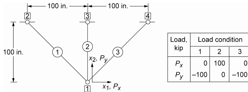
Figure 2.—Three-bar truss.
