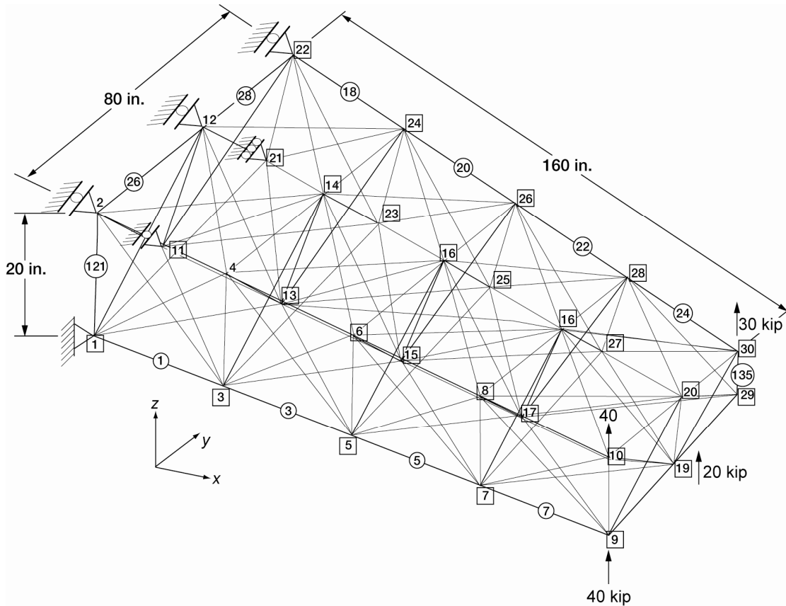
Figure 4.—Forward-swept wing.
