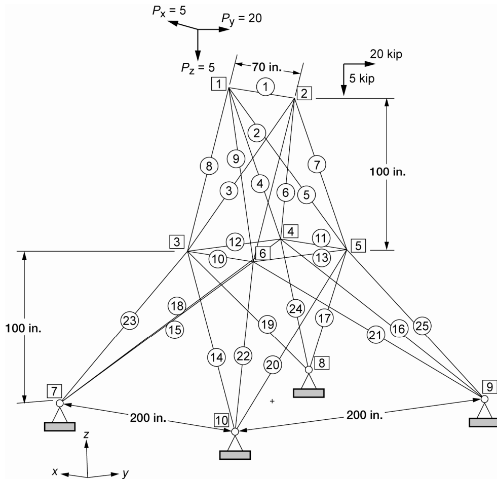
Figure 6.—Twenty-five bar tower.
