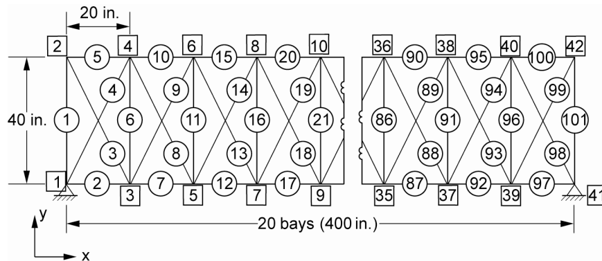
Figure 7.—Twenty-bay truss.
