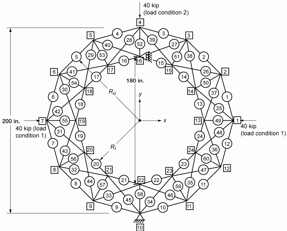
Figure 5.—Sixty-bar trussed ring.
