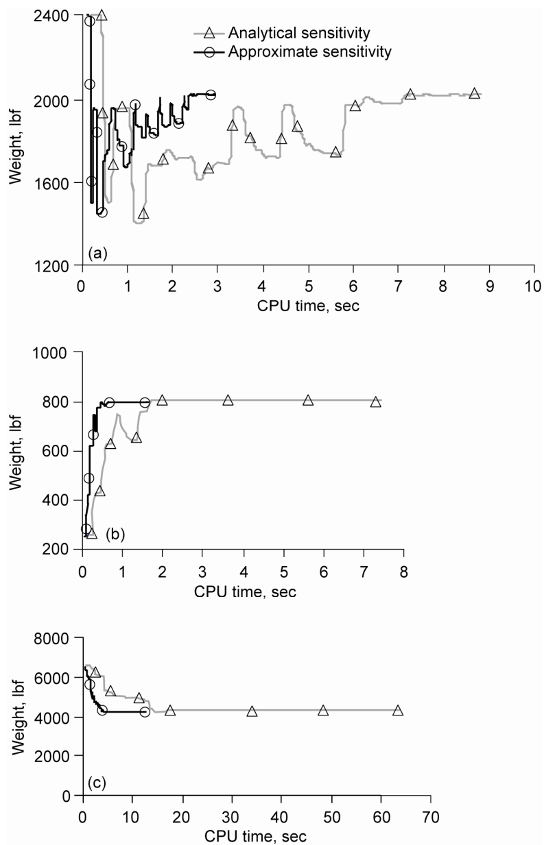
Figure 8.—CPU solution time for SQP algorithm. (a) Twenty-bay truss. (b) Sixty-bar trussed ring. (c) Forward-swept wing.
