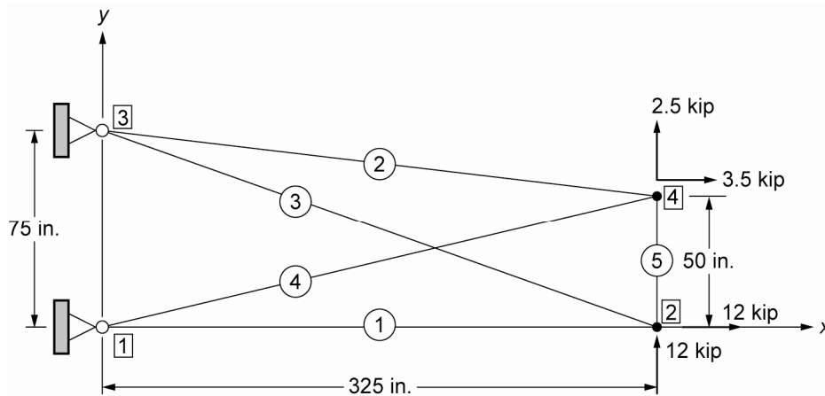
Figure 3.—Tapered five-bar truss.
