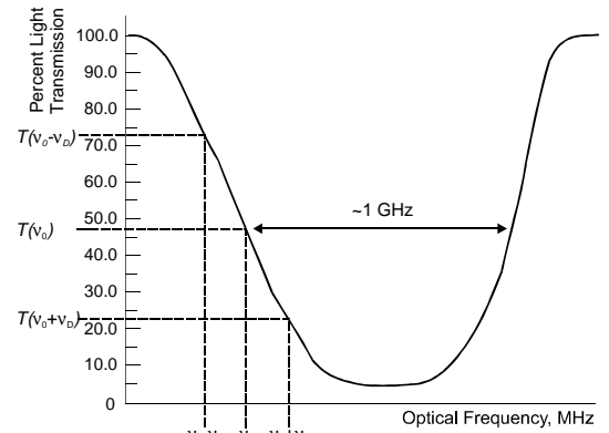
Fig. 3 IVC transfer function.
