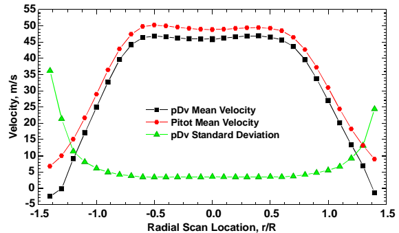
Fig. 13 Pitot probe and pDv measurements acquired at x/D = 2 with integrator and laser stabilization systems.
