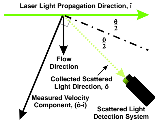
Fig. 1 DGV velocity measurement geometry.
