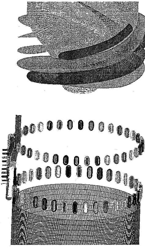
Flowliner overset grid system: 264 grid blocks of various sizes, total 66 M grid points
