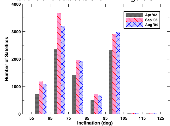
Fig. 3: Inclination distribution.
