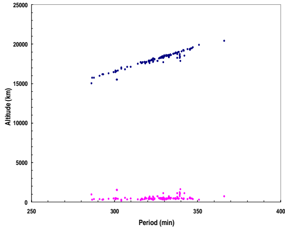
Fig. 6: Gabbard diagram of “analyst” satellites with orbital inclinations between 60° - 70° and with mean altitudes between 8,000 – 11,000 km.
