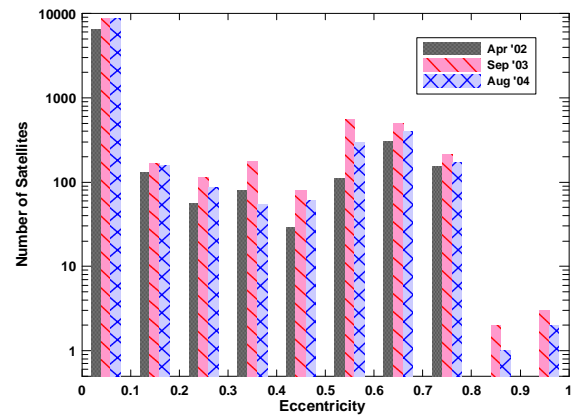
Fig. 4: Eccentricity distribution.
