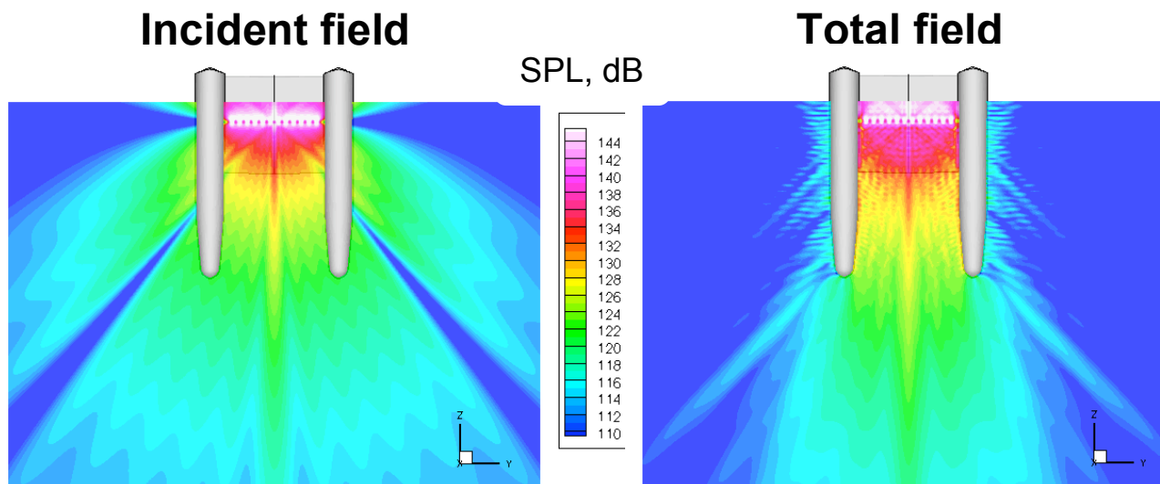
Figure 11. Incident and total sound fields (in the source plane) for twelve evenly spaced dipoles along the inboard wing at the chord location appropriate for peak jet noise from twelve engines with total power equal to that of 2 GE90-85 engines. f = 203 Hz, M = 0.3
