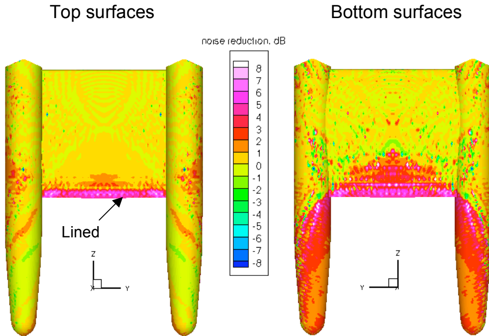
Figure 10: Noise reduction contours ( SPL_{HW} minus SPL_{LINER} ) due to acoustic liner at inboard wing trailing edge f = 316 Hz, M = 0.3 , Z = \rho c(1.0+1.5i) Incident noise generated by two monopoles above wing, 0.5\lambda apart
