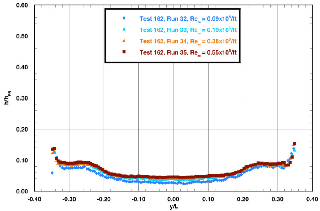
Figure C.15: RTF-BLT-PC spanwise data ( x/L = 0.85 ) in the 20-Inch \text{CF}_4 Tunnel at \alpha = 40 -deg, baseline.
