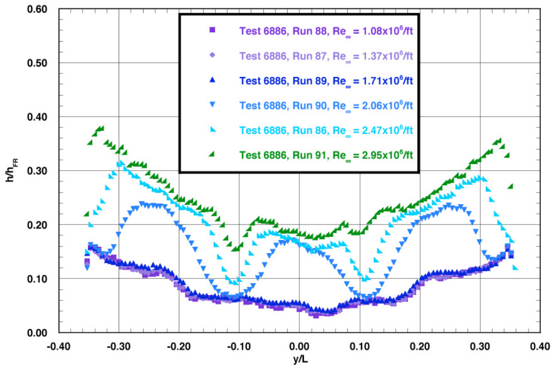
Figure A.39: RTF-BLT-P5 spanwise data ( x/L = 0.85 ) in the 20-Inch Mach 6 Air Tunnel at \alpha = 40\text{-deg} , x/L = 0.30 , k_{CL} = 0.0065\text{-in.} , k_{AL-40-INV} = 0.0065\text{-in.}
