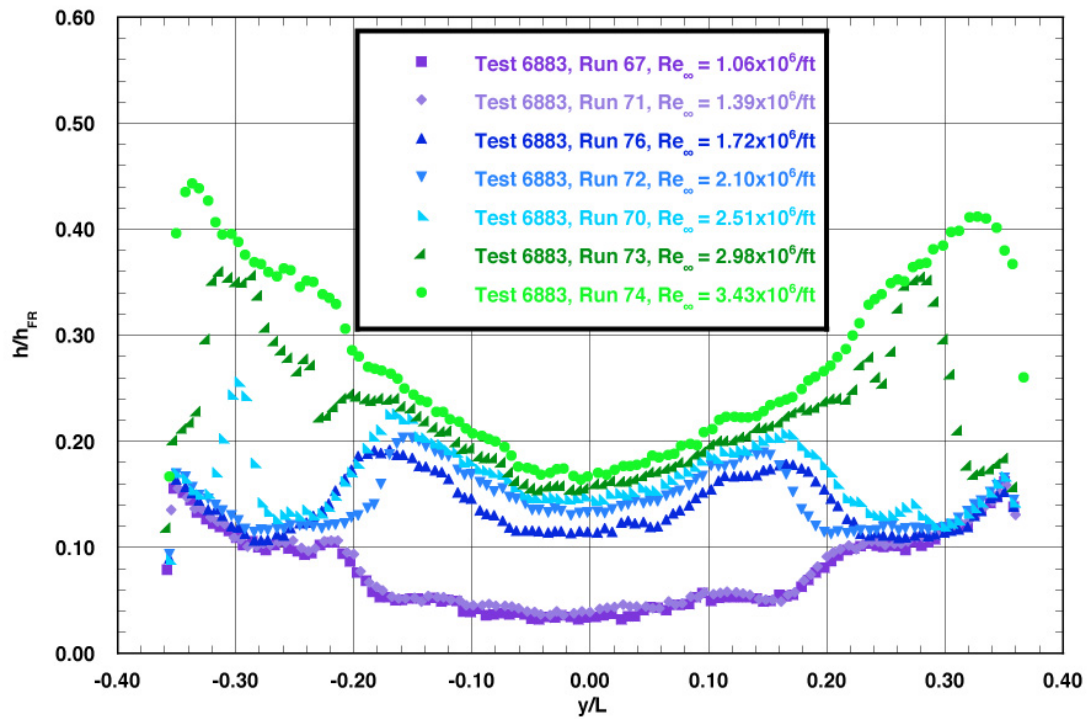
Figure A.36: RTF-BLT-P3 spanwise data ( x/L = 0.85 ) in the 20-Inch Mach 6 Air Tunnel at \alpha = 40\text{-deg} , x/L = 0.30 , k_{CL} = 0.0045\text{-in.} , k_{AL-40-VIS} = 0.0045\text{-in.}
