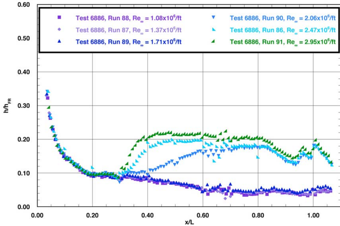
Figure A.38: RTF-BLT-P5 centerline data in the 20-Inch Mach 6 Air Tunnel at \alpha = 40\text{-deg} , x/L = 0.30 , k_{CL} = 0.0065\text{-in.} , k_{AL-40-INV} = 0.0065\text{-in.}
