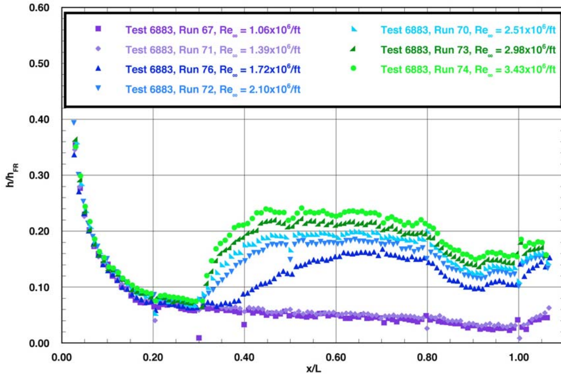
Figure A.35: RTF-BLT-P3 centerline data in the 20-Inch Mach 6 Air Tunnel at \alpha = 40\text{-deg} , x/L = 0.30 , k_{CL} = 0.0045\text{-in.} , k_{AL-40-VIS} = 0.0045\text{-in.}
