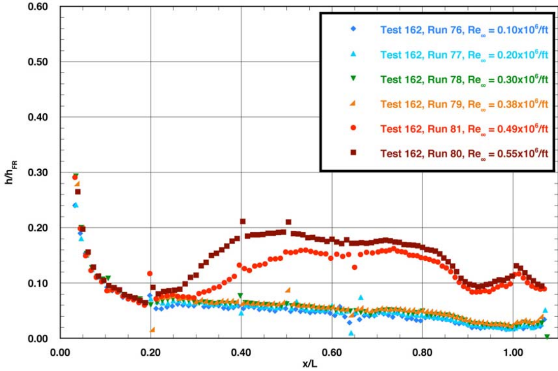
Figure C.17: RTF-BLT-PC centerline data in the 20-Inch \text{CF}_4 Tunnel at \alpha = 40\text{-deg} , x/L = 0.20 , k_{CL} = 0.0065\text{-in.} , k_{AL-40-INV+} = 0.0065\text{-in.}
