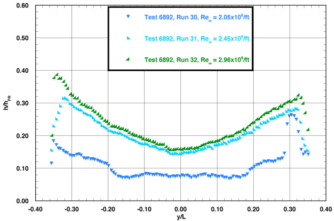
Figure A.33: RTF-BLT-PB spanwise data ( x/L = 0.85 ) in the 20-Inch Mach 6 Air Tunnel at \alpha = 40\text{-deg} , x/L = 0.10 , k_{CL} = 0.0045\text{-in.} , k_{AL-40-INV} = 0.0045\text{-in.}
