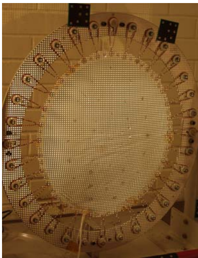
Figure 5. 0.3 meter Antenna Modified for Dot-Projection Photogrammetry.
