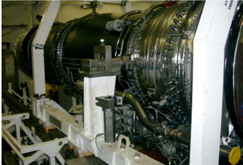
Figure 4. F/A-18 engine in repair cradle
