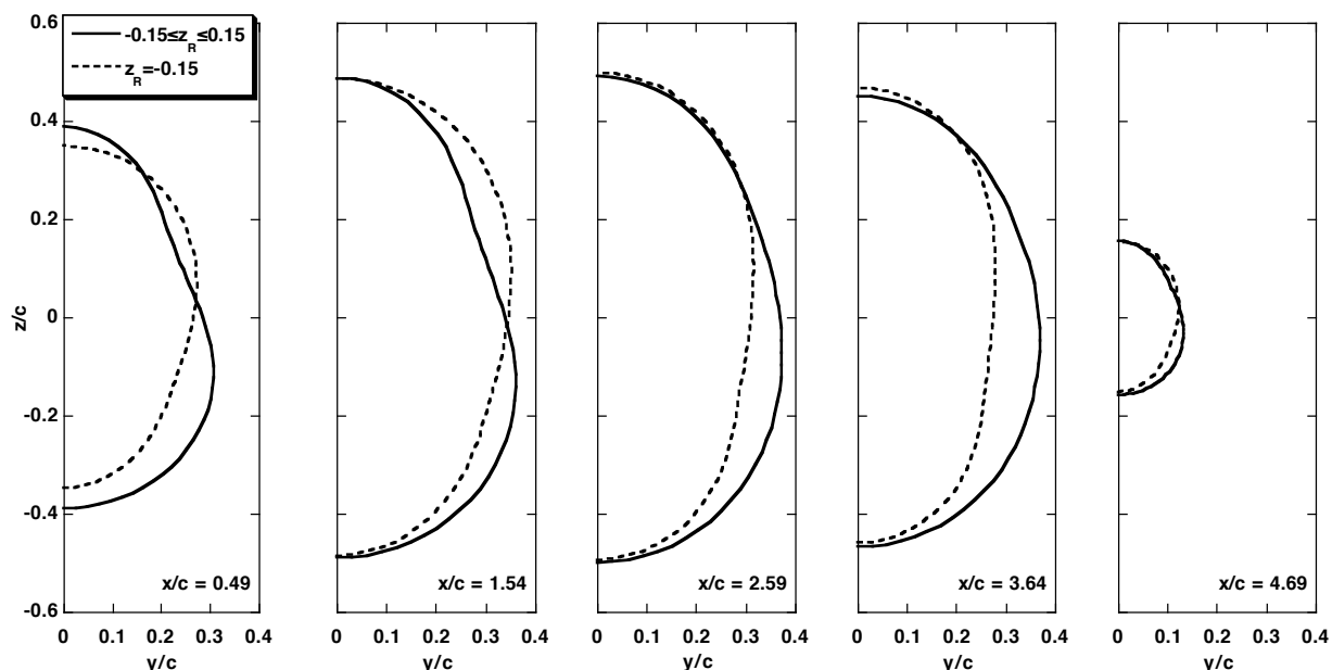
Fig. 21 Selected fuselage cross-sections for the two wing/fuselage optimization problems of Fig. 20 showing differences between the two solutions at L/D = 13 : a) baseline in which wing position is allowed to float ( -0.15 \leq z_R \leq 0.15 ) and b) wing fixed in the low-wing position ( z_R = -0.15 ): C_L = 0.45 , M_\infty = 0.84 , ISELECT = 4, ITRAN = 0, N_O = 2 , N_C = 66 , N_G = 43/42 , \beta = 0.1 , p_1 = 0.2 , p_2 = 0.2 , and P = (0.02, 0.33, 0.33, 0.32) .
