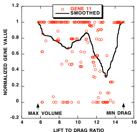
a) x -location of airfoil maximum thickness on lower surface at wing tip, GENE_{11} = x_{l0_2} .
