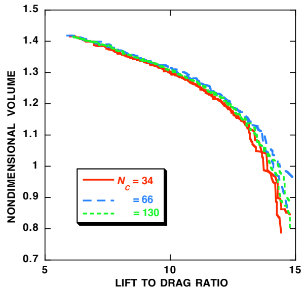
Fig. 17 Pareto front comparisons for three population sizes, each with two different ISEED values: C_L = 0.45 , M_\infty = 0.84 , ISELECT = 4 , ITRAN = 0 , N_O = 2 , N_G = 43 , \beta = 0.1 , p_1 = 0.2 , p_2 = 0.2 .
