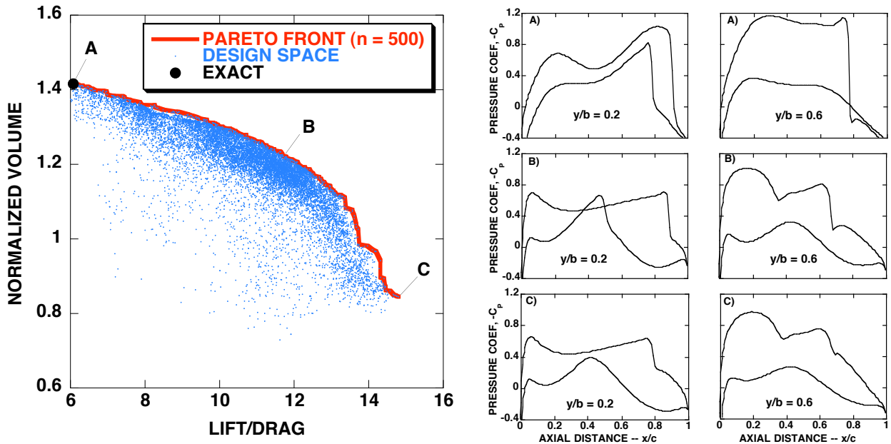
Figure 12: Design space for wing-body two-point optimization problem: C_L = 0.45 , M_\infty = 0.84 , ISELECT = 4, ITRAN = 0, N_O = 2 , N_C = 34 , N_G = 43 . Wing sectional pressures at three positions along Pareto front: A) max volume, B) intermediate, C) min drag.
