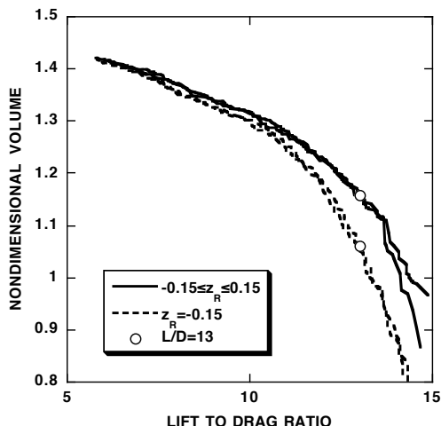
Fig. 20 Pareto front comparisons for two different wing-fuselage optimization cases: a) baseline in which wing position is allowed to float ( -0.15 \leq z_R \leq 0.15 ) and b) wing fixed in the low-wing position ( z_R = -0.15 ). Each computation performed with two ISEED values: C_L = 0.45 , M_\infty = 0.84 , ISELECT = 4, ITRAN = 0, N_O = 2 , N_C = 66 , N_G = 43/42 , \beta = 0.1 , p_1 = 0.2 , p_2 = 0.2 , and P = (0.02, 0.33, 0.33, 0.32) .
