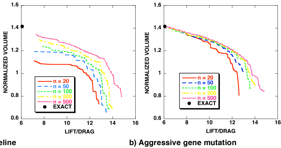
Figure 11: Pareto front convergence for wing-body optimization involving drag minimization and volume maximization: C_L = 0.45 , M_\infty = 0.84 , ISELECT = 4, ITRAN = 0, N_O = 2 , N_C = 34 , N_G = 43 .
