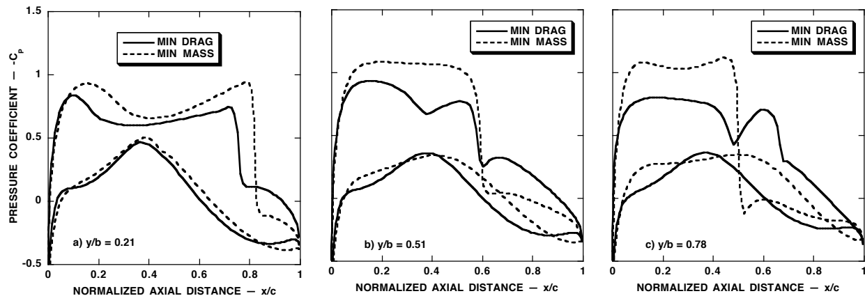
Fig. 9 Pressure coefficient distributions at selected spanwise stations for the wing optimization problem presented in Fig. 8 showing differences between the two Pareto front endpoints: ISELECT = 3, ITRAN = 0, M_\infty = 0.84 , C_L = 0.45 , N_C = 32 , N_G = 22 , \beta = 0.1 , p_1 = 0.2 , p_2 = 0.2 and P = (0.04, 0.32, 0.32, 0.32) .
