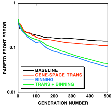
Fig. 7 Average convergence history curves for GA variations plotted in Figs. 4 and 5: M_\infty = 0.84 , C_L = 0.45 , N_C = 32 , N_G = 22 , \beta = 0.1 , p_1 = 0.2 , p_2 = 0.2 and P = (0.04, 0.32, 0.32, 0.32) .
