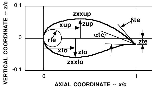
Fig. 1 Airfoil parameterization used for each wing defining station (taken from Sobieczky 46 ). Angles are measured in degrees. All lengths are nondimensionalized by wing-root chord.
