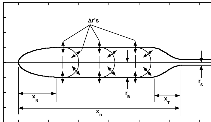
Fig. 2 Sketch showing decision variable definitions for the fuselage parameterization. For this arrangement there are three axial stations ( N_x = 3 ) and four circumferential stations ( N_T = 4 ).
