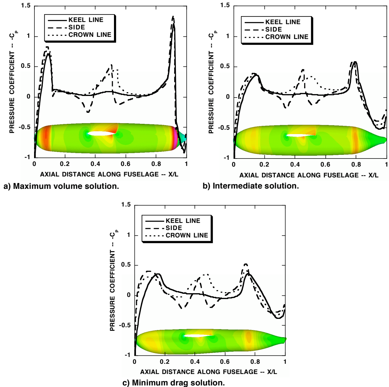
Fig. 14 Fuselage pressure distributions for the wing/body optimization problem presented in Fig. 12 at three positions along the Pareto front.
