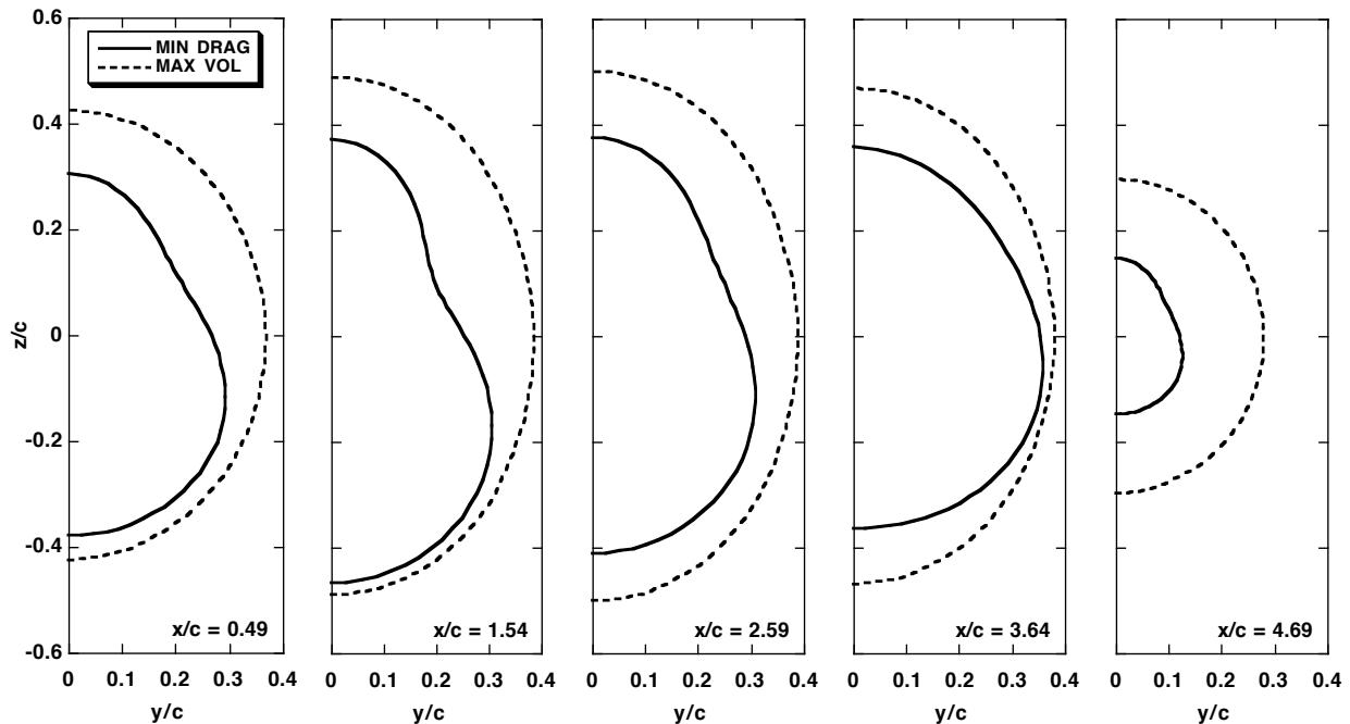
Fig. 15 Selected fuselage cross-sections for the wing/fuselage optimization problem of Fig. 12 showing differences between two Pareto front endpoints: C_L = 0.45 , M_\infty = 0.84 , ISELECT = 4, ITRAN = 0, N_O = 2 , N_C = 34 , N_G = 43 , \beta = 0.1 , p_1 = 0.2 , p_2 = 0.2 and P = (0.04, 0.32, 0.32, 0.32) .
