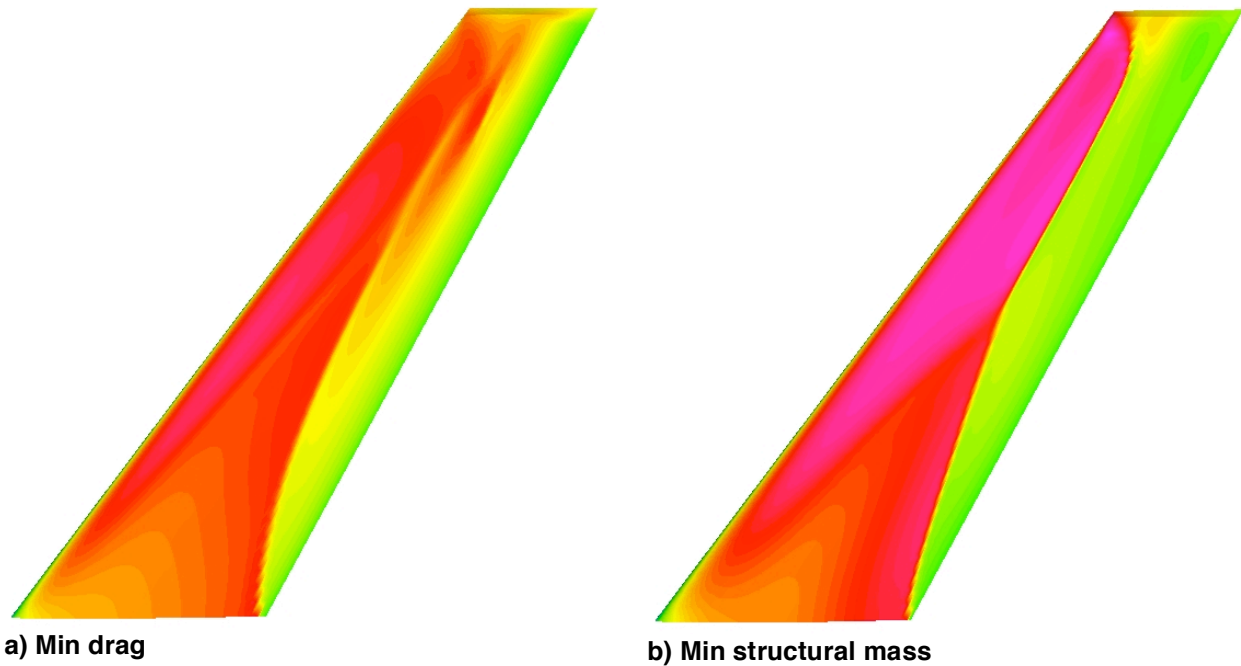
Fig. 8 Upper surface Mach number contours for transonic wing optimization in which drag at fixed lift and structural mass are simultaneously minimized: ISELECT = 3, ITRAN = 0, M_\infty = 0.84 , C_L = 0.45 , N_C = 32 , N_G = 22 , \beta = 0.1 , p_1 = 0.2 , p_2 = 0.2 and P = (0.04, 0.32, 0.32, 0.32) .
