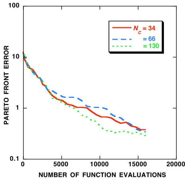
Fig. 16 Pareto front convergence history comparisons for three population sizes, each averaged over two ISEED values: C_L = 0.45 , M_\infty = 0.84 , ISELECT = 4 , ITRAN = 0 , N_O = 2 , N_G = 43 , \beta = 0.1 , p_1 = 0.2 , p_2 = 0.2 .
