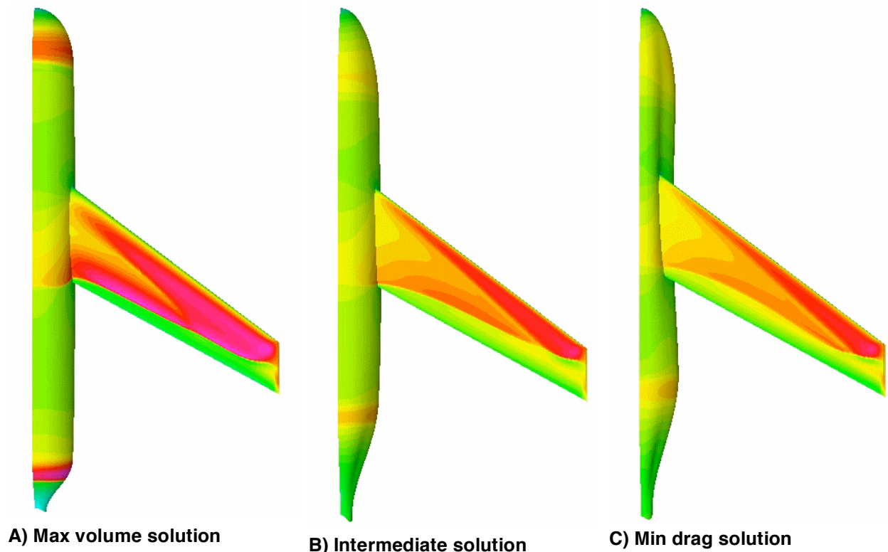
Fig. 13 Surface Mach number contours for the wing/body optimization problem presented in Fig. 12 at three positions along the Pareto front.
