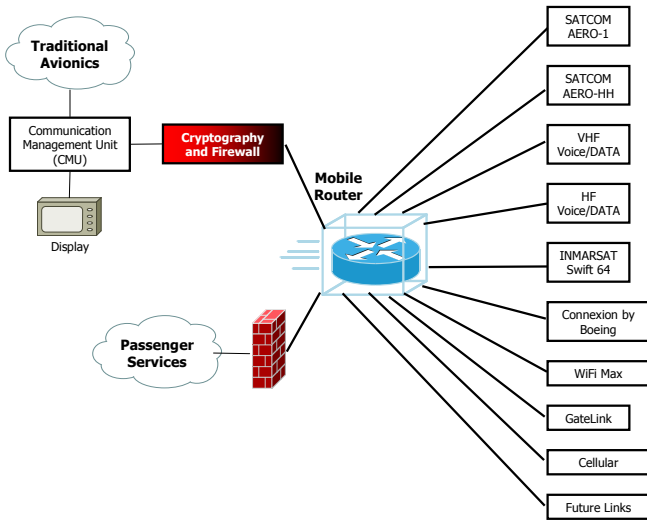
Figure 4.—IP-based transitional architecture.
