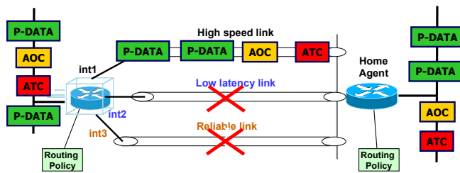
Figure 7.—Policy-based routing, passenger link active.
