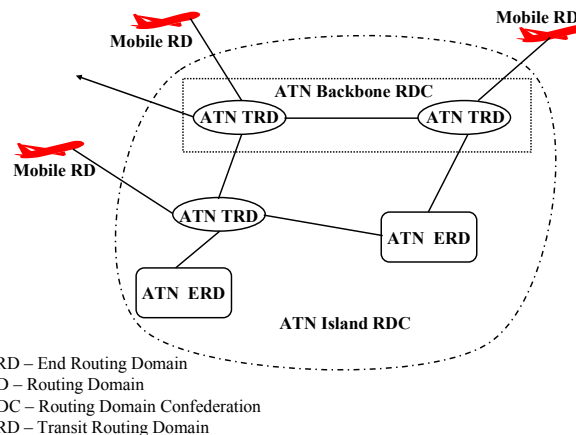
Figure 3.—ATN Island routing domain confederation.
