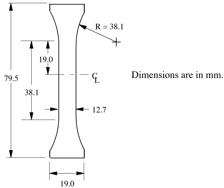
Figure 7. Diagram of dog-bone shaped compression specimen for ASTM D695-96 tests.
