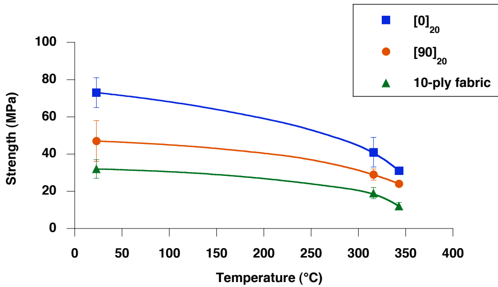
Figure 13. Interlaminar shear strength from ASTM D-3846 tests.
