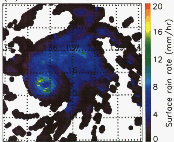
(e) BAYESIAN-MLE
