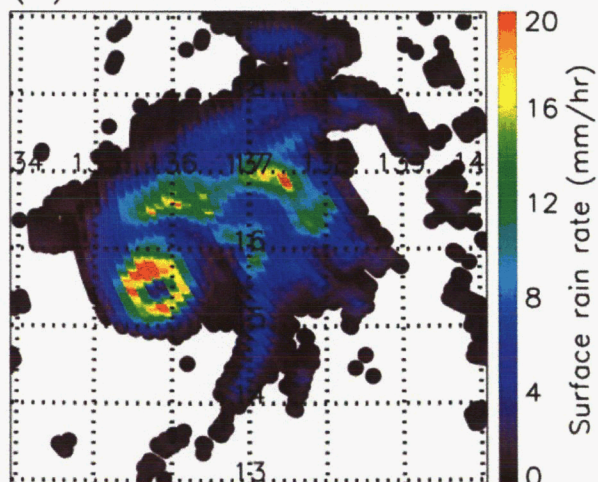
(e) BAYESIAN-MLE
