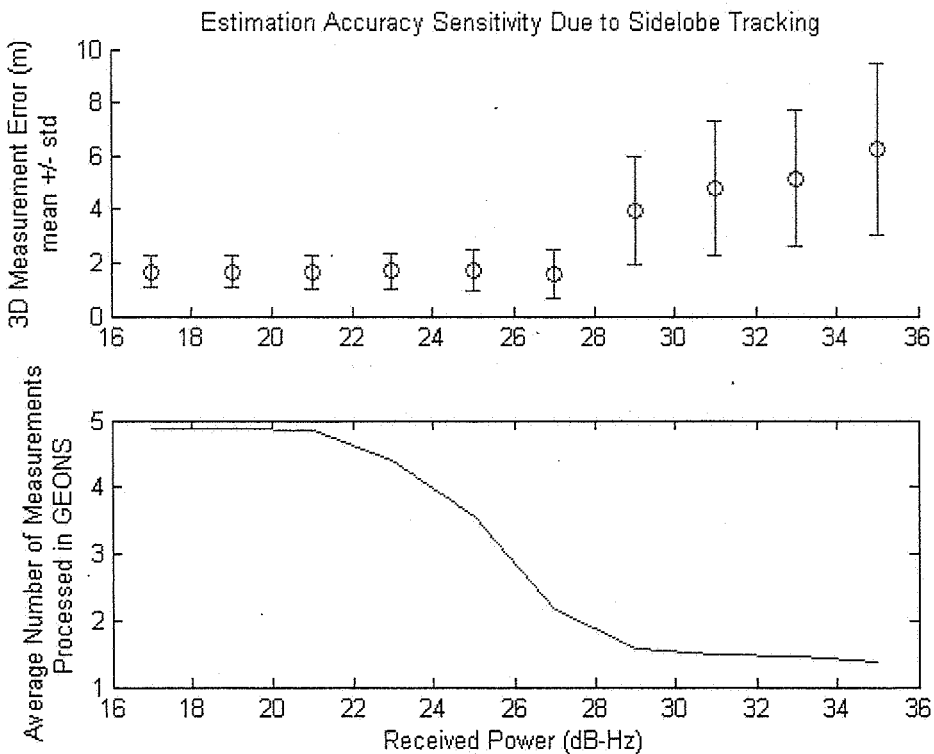
Figure 7 - Sensitivity to receiver acquisition/tracking threshold
