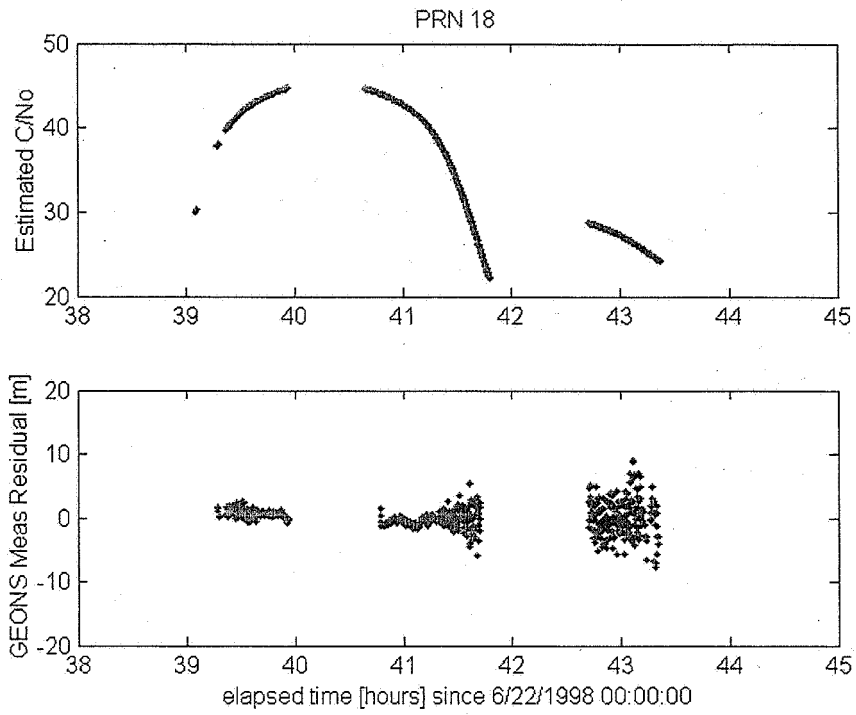
Figure 10 - Variation in Receiver Measurement Noise with C/No
