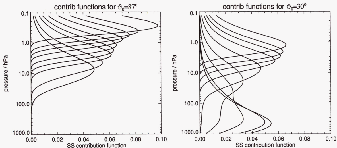
Figure 2. Sample contribution functions for SBUV channels at different SZA for a typical ozone profile (267 DU). Displayed is the single scattering (SS) contribution to the measured radiance, normalized to total radiance: (\delta I_{SS})/(\delta p)(I_{SS}/I_0) . The channel wavelengths in nm, from top to bottom are 274, 283, 288, 292, 298, 302, 306, 313 and 318. (Plot adapted from Figure 2 in [Bhartia et al. , 1996])
