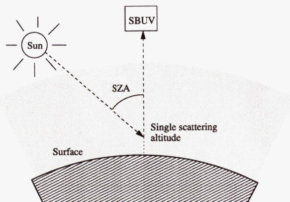
Figure 1. Sketch of the observation geometry.
