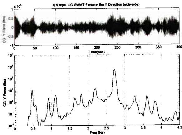
Figure 4. CG SWAT Force in the Y Direction (Lateral)
