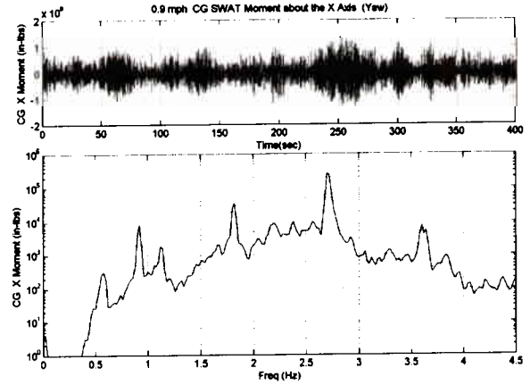
Figure 6. CG SWAT Moment about X (Yaw)
