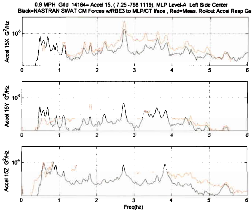
Figure 11. NASTRAN Results With SWAT Force Inputs (Black) vs. Measured Accelerations (Red) – X, Y, Z @ Left Side of MLP
