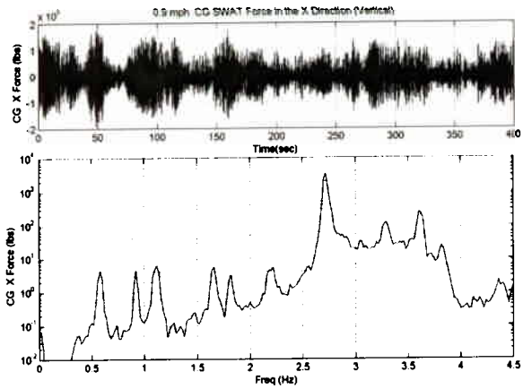
Figure 3. CG SWAT Force in the X Direction (Vertical)
