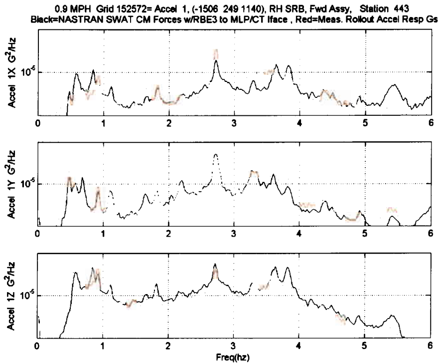
Figure 12. NASTRAN Results With SWAT Force Inputs (Black) vs. Measured Accelerations (Red) – X, Y, Z @ Top of Right SRB
