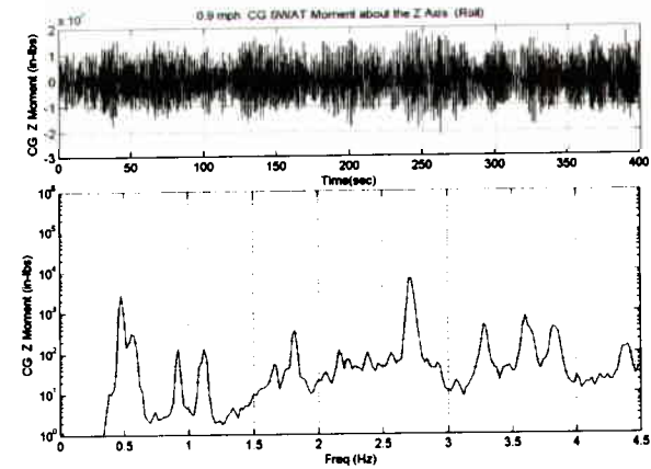
Figure 8. CG SWAT Moment about Z (Roll)
