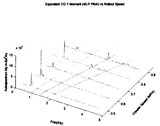
Figure 17. SWAT CG YY Moment (Pitch) vs. Speed
