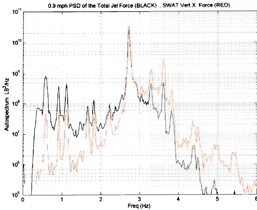
Figure 10. SWAT X Force (Red) and Sum of All JEL Forces as Estimated from Pressures (Black) – Frequency Domain
