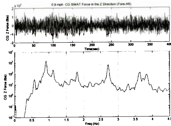
Figure 5. CG SWAT Force in the Z Direction (Travel)
