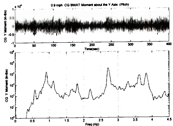
Figure 7. CG SWAT Moment about Y (Pitch)
