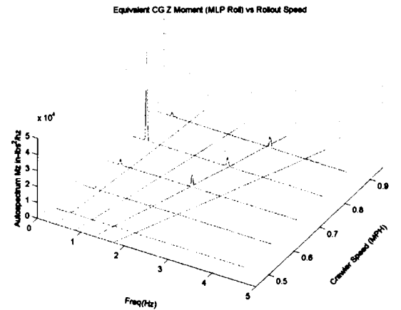
Figure 18. SWAT CG ZZ Moment (Roll) vs. Speed
