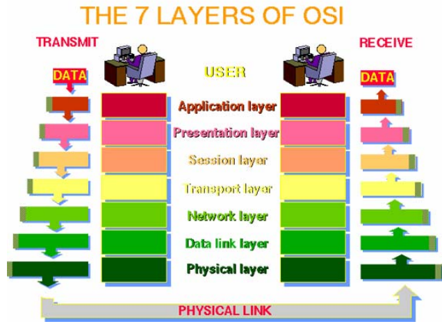
Fig. 4. OSI layers [7]
