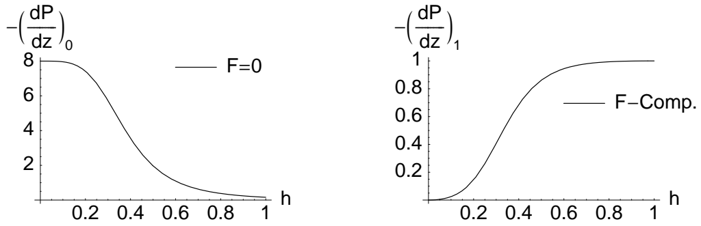
Figure 16: The purely viscous ( (dp/dz)_0 \equiv dp/dz for F = 0 ) and gravitational (the coefficient of F in eq. 58) components of the pressure gradient. M = 0.02 . To get dp/dz for arbitrary F one should add (dp/dz)_0 + F (dp/dz)_1 .
