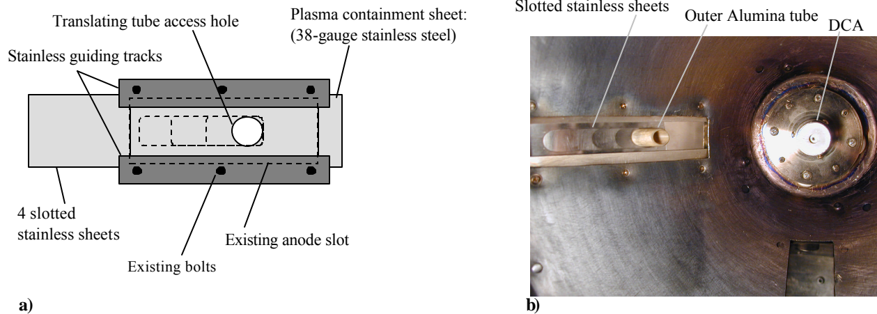
Figure 2. Schematic of the discharge plasma containment hardware covering the anode side slot shown in a), along with a photograph taken inside the FMT2 discharge chamber prior to engine testing showing the interior of the discharge plasma containment mechanism in b).
