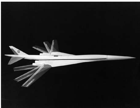
Time-lapse photography shows the variable sweep wing of early Boeing Model 733-290 Supersonic Transport design. Free-flight testing was conducted in the Langley Full-Scale Tunnel.
