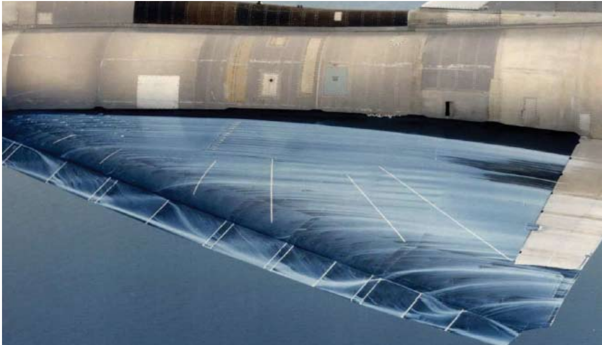
Surface-oil studies illustrate multiple vortex flows seen on the leading edge.
