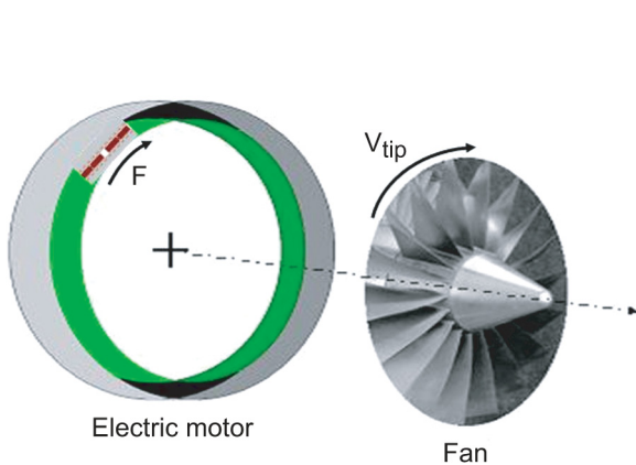
Figure 18.—Tip-drive motor to fit around propulsive fan.
