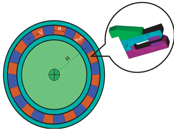
Figure 19.—Rotor permanent magnet arrangement for tip-drive motor.
