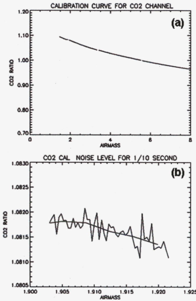
Figure 8. In (a), the CO 2 ratio from ground measurements on May 13, 2004 is calibrated to the airmass. Enlargements of noise for data taken at 1/10 second is shown in (b) with a ten point average shown as a solid line.
