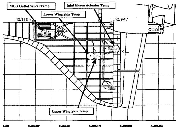
Figure 3. Left Wing Temperature Sensors used in Columbia Ascent Analysis
