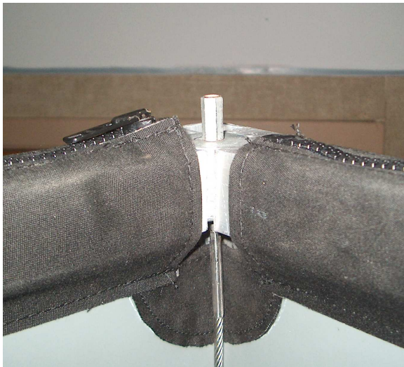
Figure 3: Corner detail.
