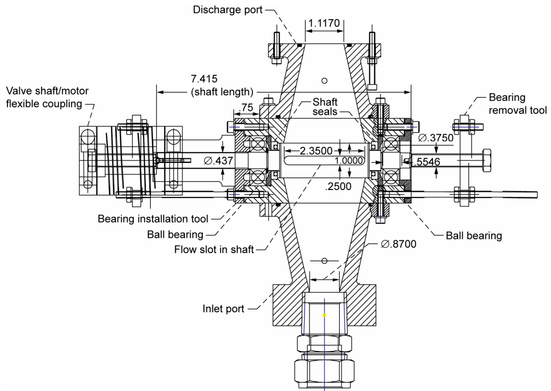
Figure 3.—Pulsation valve assembly cross section.
