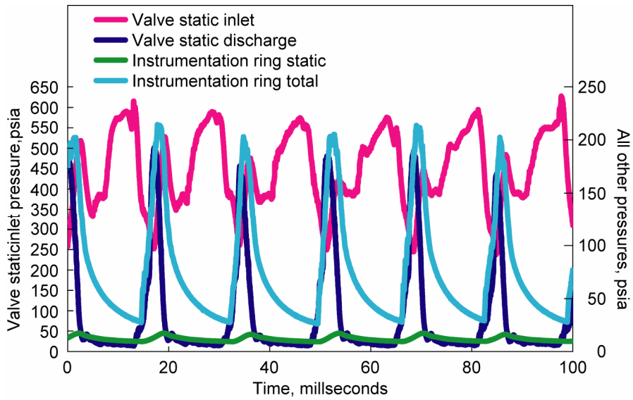
Figure 13.—Pulsation valve pressure test data, 1800 rpm, 60 Hz.
