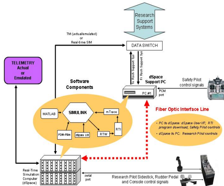
Figure 15. FDM-PSIM Configuration
