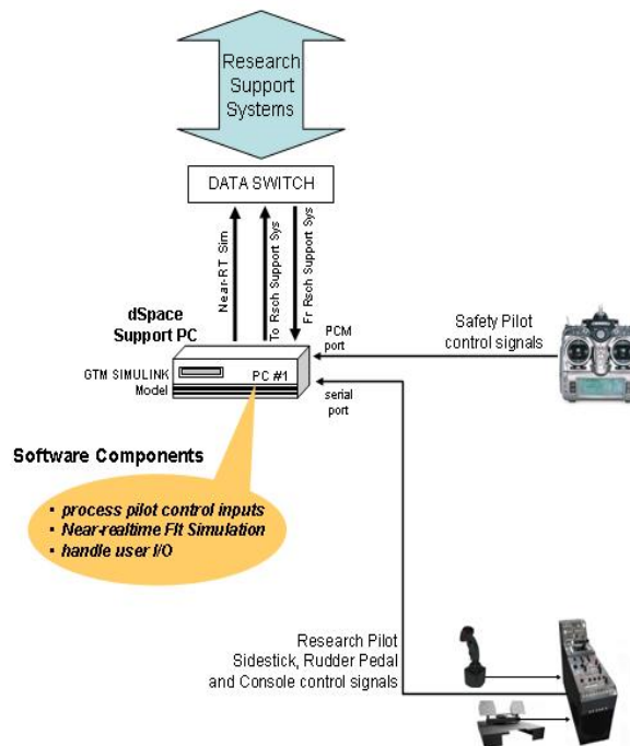
Figure 14. FDM-PC Configuration
