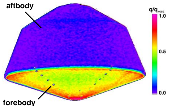
Heating on Notional Mars Entry Vehicle Geometry
