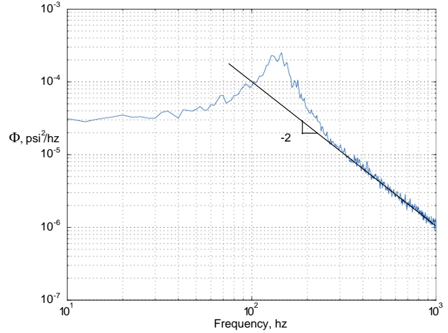
Figure 4. Buffet Pressure PSD from JSF model data at AOA of 22 degrees.
