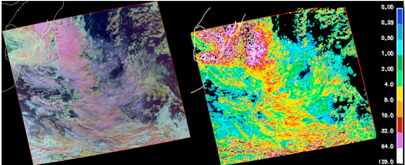
Figure 1: CERES imagery for multilayer cloud detection comparisons for 1316 UTC, 13 July 2004. left: Aqua MODIS pseudo-color RGB image. right: VISS-derived cloud optical depth.
