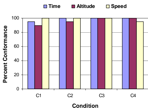
Figure 12. Ames Subject Pilot Meter Fix Conformance
