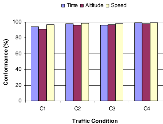
Figure 16. Overall Meter Fix Conformance
