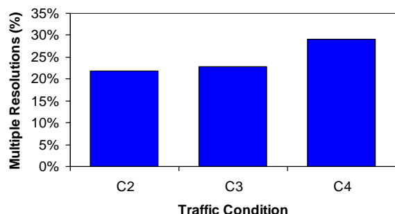
Figure 6. Conflicts Requiring Multiple Resolution Maneuvers (Pilot-Resolved Scripted Conflicts)
