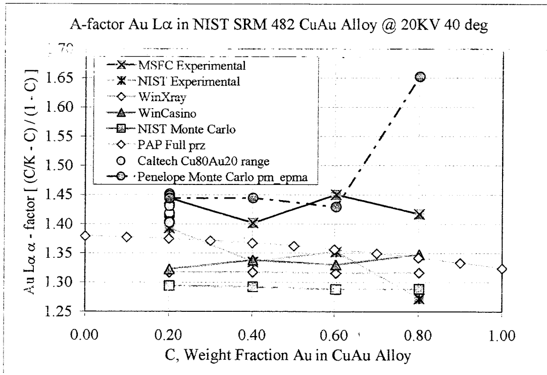
Figure 2 Au L \alpha \alpha -factors in CuAu binary using NIST SRM 482 CuAu compositions.
