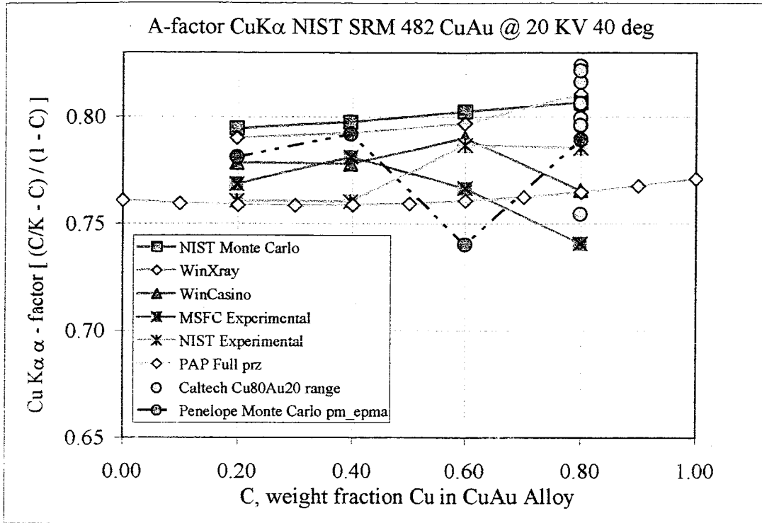
Figure 1 Cu K \alpha \alpha -factors in CuAu binary using NIST SRM 482 CuAu compositions. Calculated data values using NIST, WinXray, WinCasino, and Penelope Monte Carlo algorithms, compared with PAP full \phi(\rho z) calculated values, and experimental EPMA data from NIST, Caltech, and Marshall microprobes. Range of typical replicate measurements indicated for Caltech Cu 80 Au 20 alloy; compare with range for EPMA measurements.
