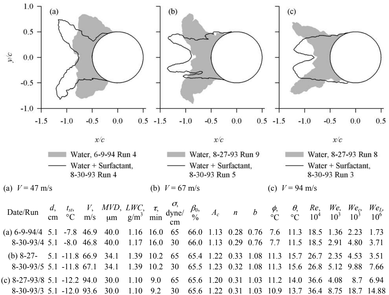
Figure 1. Effect of Surfactant and Velocity on Ice Shape. Vertical Cylinders Tested in the NASA Glenn IRT. Published and Unpublished Ice-Shape Data from Tests by Bilanin and Anderson.
