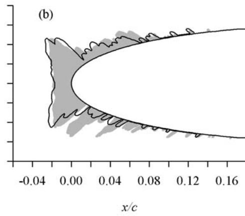
(b) Model Chord Scaled from 91 to 53 cm; n , 0.4.
