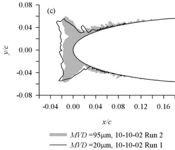
(c) MVD , 95 and 20\mu\text{m} ; c , 91.4 cm; V , 77 m/s; n , 0.3
