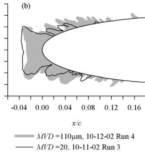
(b) MVD , 110 and 20\mu\text{m} ; c , 53.3 cm; V , 51 m/s; n , 0.5.
