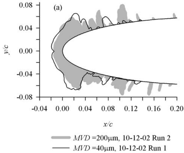
(a) MVD , 200 and 40\mu\text{m} ; c , 53.3 cm; V , 51 m/s; n , 0.3.
