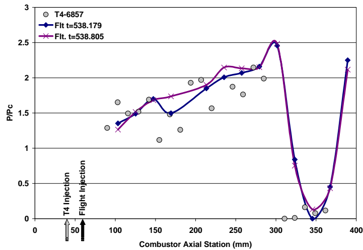
Figure 17. Flight-to-ground comparison for the fueled combustor at windward conditions
