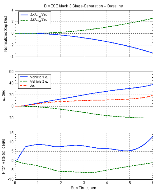
Figure 19. Mach 3 baseline separation.
