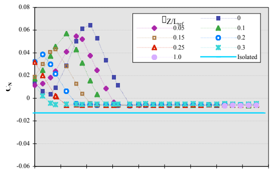
Figure 12: Variation of bimese-orbiter static normal force coefficient with x/L_{ref} and z/L_{ref} at Mach 3 for \alpha = 0 , \beta = 0 degrees.
