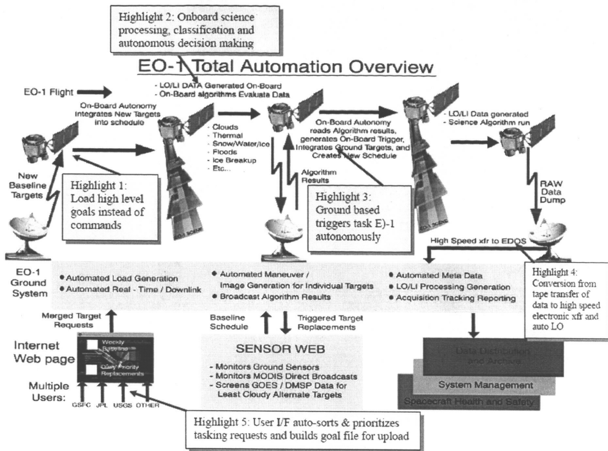
Figure 3 Overview of autonomy and automation software installed on the EO-1 mission
