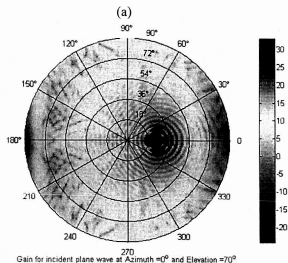
Gain for incident plane wave at Azimuth = 0^\circ and Elevation = 70^\circ
