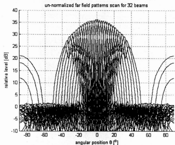
Fig. 3. Scan loss and un-normalized radiation pattern for 32 beams. Scalloping loss is better than 1.6dB (worst case).
