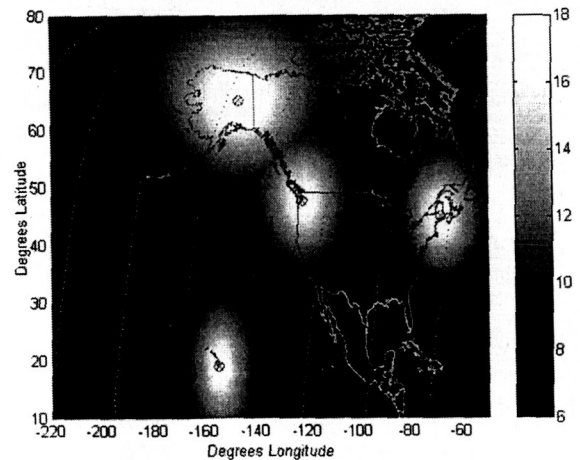
Fig. 11. Received signal strength as a function of the sub-satellite point for four downlink stations, located in Hawaii, Washington, and Maine. The shading scale range is different than Fig. 5 to enhance readability.
