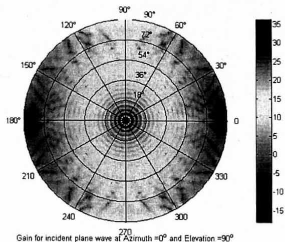
Gain for incident plane wave at Azimuth = 0^\circ and Elevation = 90^\circ
