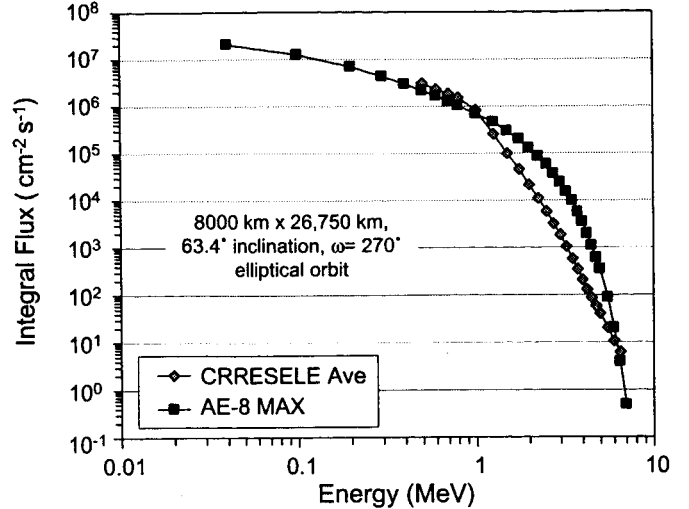
Fig. 7. CRRESELE Average model versus AE-8 MAX at solar maximum for an 8000 km x 26,750 km, 63.4° inclination, \omega=270^\circ , elliptical orbit.
