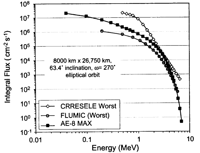
Fig. 8. Worst-case electron models versus AE-8 MAX at solar maximum for an 8000 km x 26,750 km, 63.4° inclination, \omega=270^\circ , elliptical orbit.
