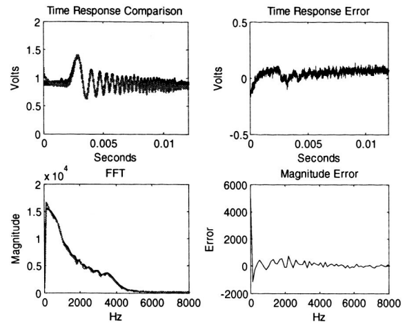
Figure 10 Time and frequency response comparison with sine sweep input and inverted second stage evolved transfer function output
