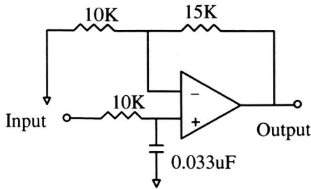
Figure 5 Simulated Analog Plant
