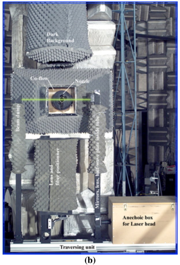
Figure 3.—Photographs of the jet facilities; (a) 1" unheated jets, (b) 2" heated jets.
