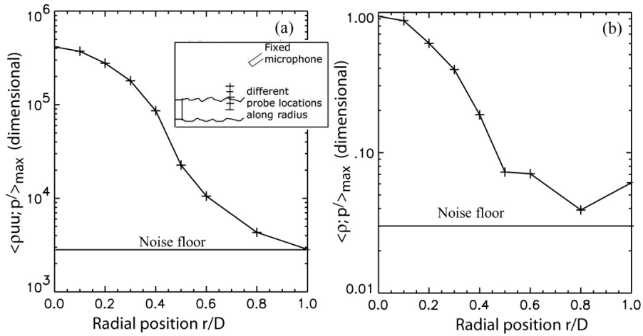
Figure 11.—Maximum value of correlation between sound fluctuations at fixed microphone ( \theta_p = 150^\circ , R/D = 50 ) and (a) \rho uu and (b) \rho fluctuations from various radial positions at x/D = 10 inside unheated M_a = 1.18 jet. Note that correlation values are not normalized.
