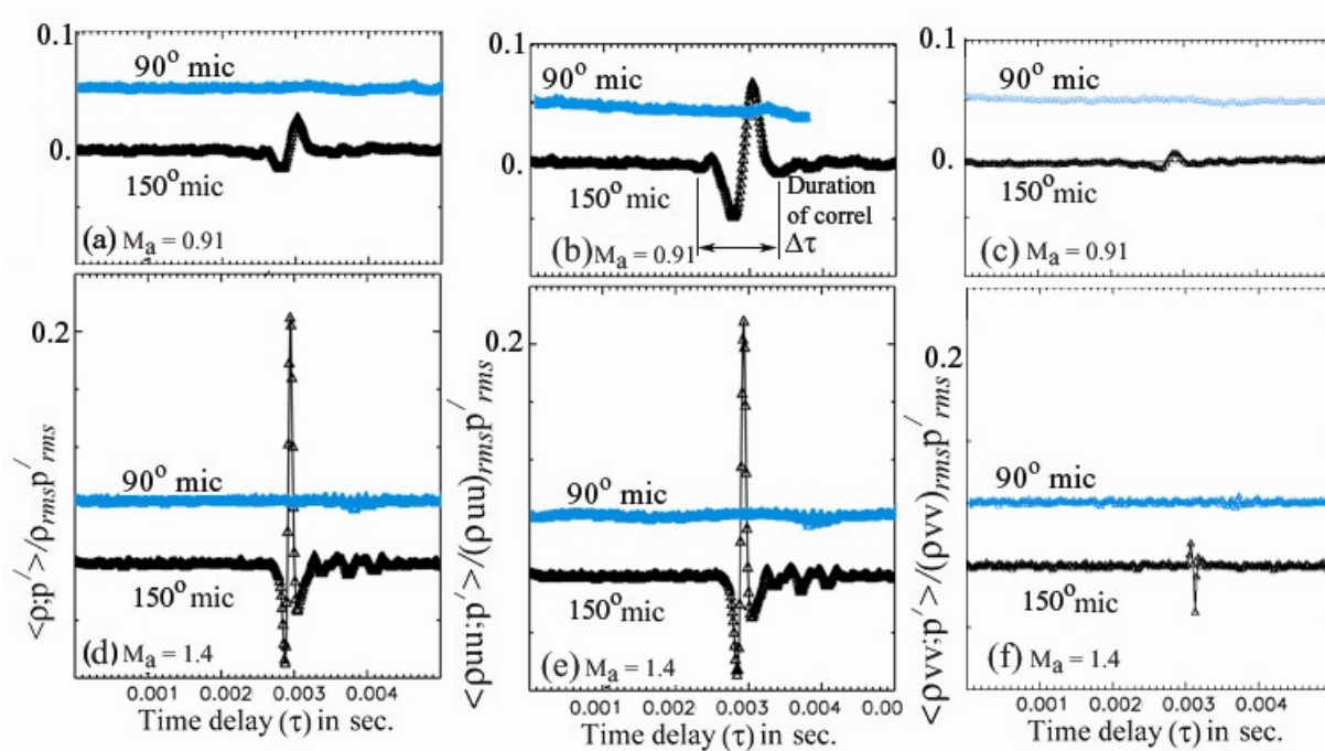
Figure 4.—Normalized cross-correlation between sound pressure fluctuations p' and (a), (d) air density \rho ; (b), (e) \rho_{uu} ; (c), (f) \rho_{vv} fluctuations measured in M_a = 0.91 and 1.4 jets. For (a), (b), and (c) laser probe was at x/D = 10 and centerline; for (d) and (e) probe is at x/D = 12 and centerline; for (f) it is x/D = 6 and r/D = 0.48 . The microphone was kept at 50D and at indicated polar angles. The 90^\circ microphone data are shifted by 0.05.
