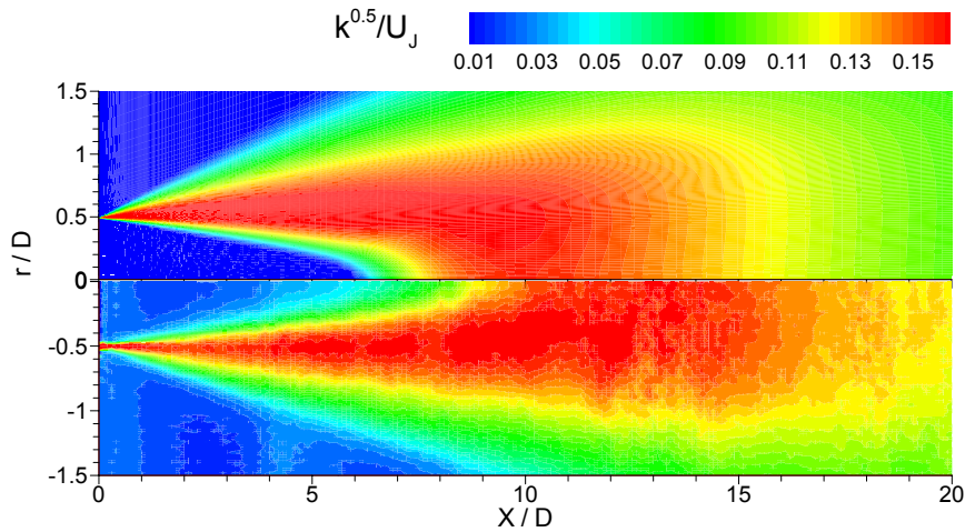
Figure 12(b).—Distribution of turbulent kinetic energy (SP07). Top half, RANS prediction; bottom half, PIV measurements.
