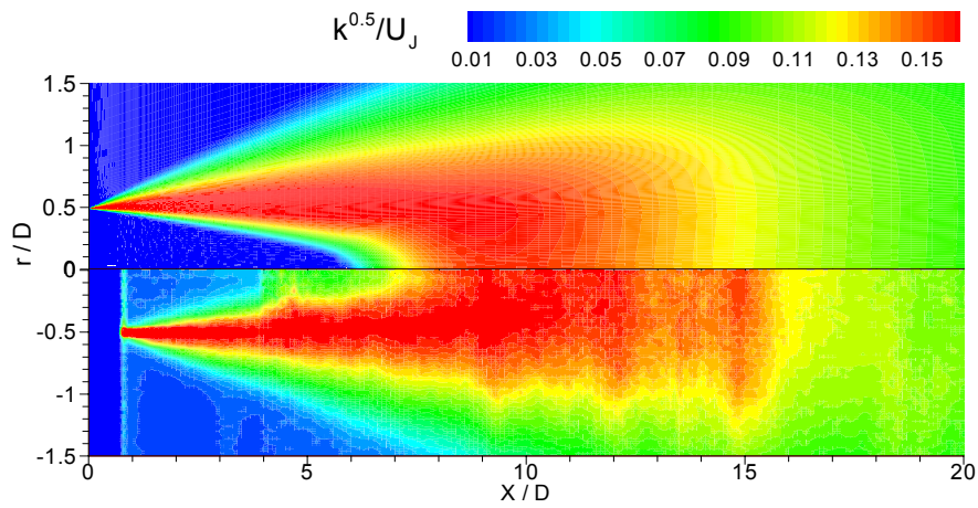
Figure 12(a).—Distribution of turbulent kinetic energy (SP03). Top half, RANS prediction; bottom half, PIV measurements.
