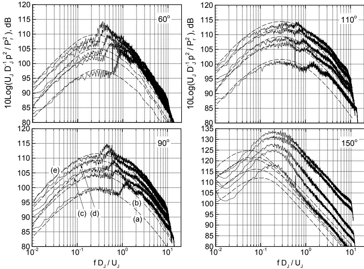
Figure 7(b).—Comparison between calculated spectra and data at indicated inlet angles at r/D_j = 100 . (a) M_j = 1.185 , (b) M_j = 1.40 , (c) M_j = 1.50 , (d) M_j = 1.66 , (e) M_j = 1.80 .
