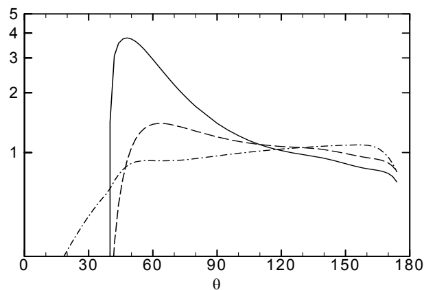
Figure 8(a).—Directivity \Lambda(\bar{x}, \bar{x}^s, \omega) due to a stationary ring source in Mach 0.9, T_r = 2.78 jet at St = 0.10 , x_1^s/D_j = 7.5 and r^s/D_j : 0.0 (solid line); 0.50 (dashed line); 2.0 (dash-dot).
