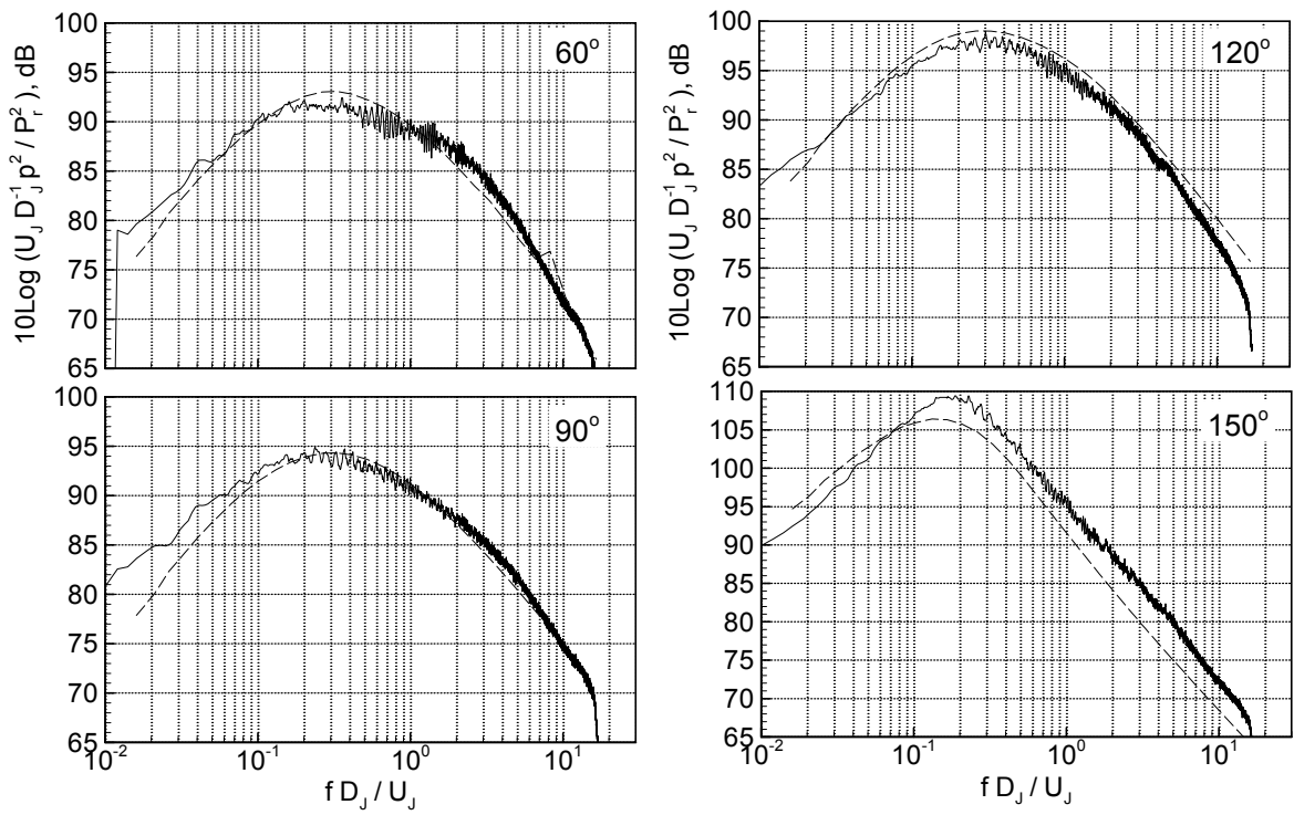
Figure 6.—Spectra in Mach 0.51, T_r=1.0 (SP03) jet at indicated inlet angles and at R/D_j = 100 .
