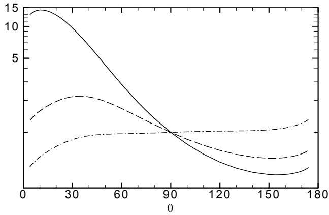
Figure 3(a).—Directivity D(\bar{x}, \bar{x}^s, \omega) due to a stationary ring source in a Mach 0.9 unheated jet at St = 0.10 , x_i^s/D_j = 7.5 and r^s/D_j : 0.0 (solid line); 0.50 (dashed line); 2.0 (dash-dot).
