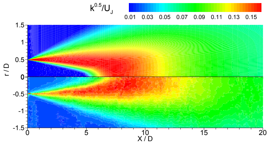
Figure 12(c).—Distribution of turbulent kinetic energy (SP49). Top half, RANS prediction; bottom half, PIV measurements.
