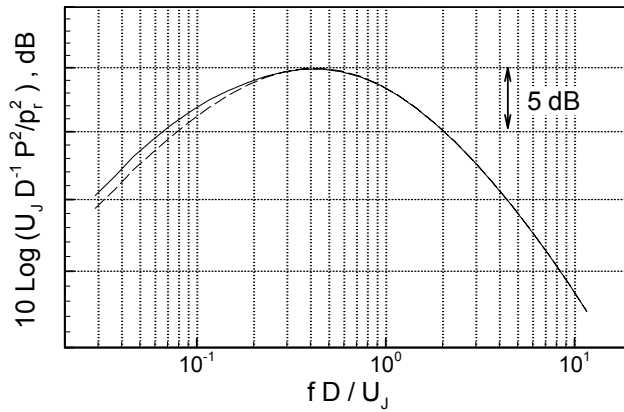
Figure 10.—Far-field spectrum at 90^\circ in a Mach 0.801, T_r = 3.0 jet. Exact Green's function (solid line); density-scaled GF (dashed line).
