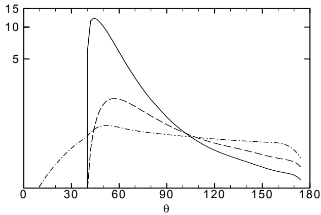
Figure 9(a).—As figure 8(a) but for a convecting ring source at observer St = 0.10 .
