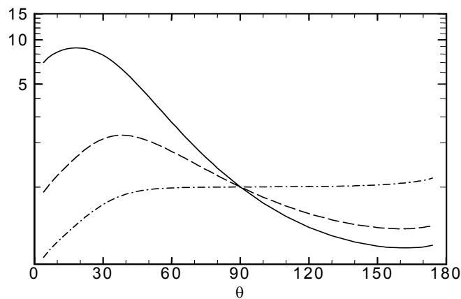
Figure 2(a).—Directivity D(\bar{x}, \bar{x}^s, \omega) due to a stationary ring source in a Mach 0.9 unheated jet at St = 0.10 , x_1^s/D_j = 1.0 and r^s/D_j : 0.0 (solid line); 0.50 (dashed line); 1.0 (dash-dot).
