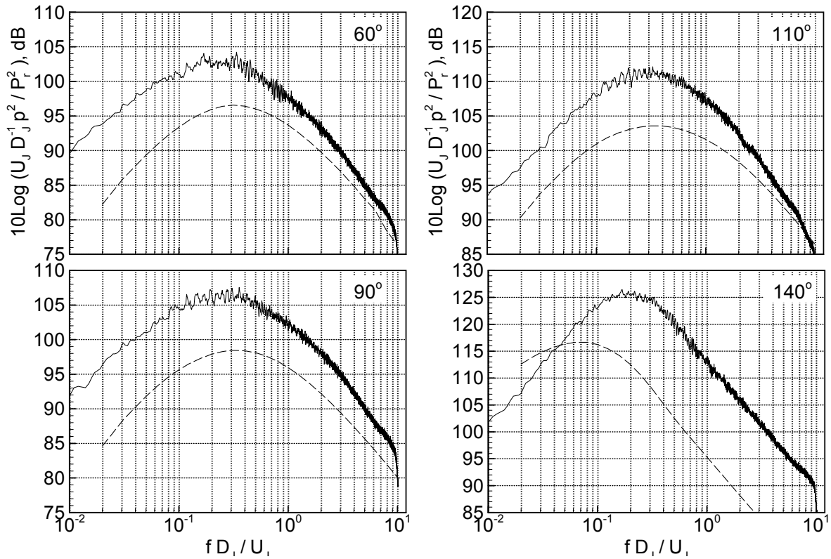
Figure 11.—Spectra in Mach 0.90, T_r = 3.14 (SP49) jet at indicated inlet angles and at R/D_j = 100 .
