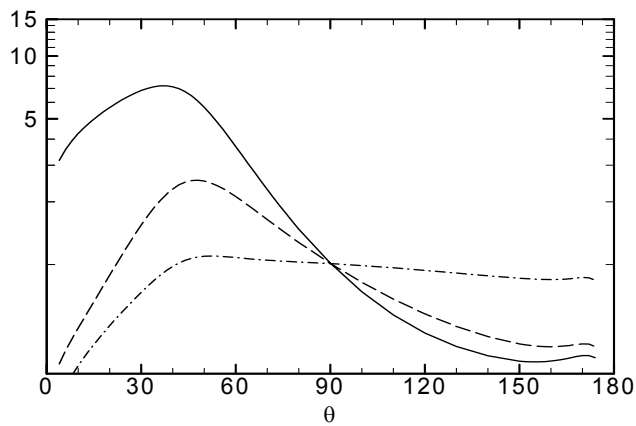
Figure 4.—Directivity D(\bar{x}, \bar{x}^s, \omega) due to a convecting ring source in a Mach 0.9 unheated jet at observer St = 0.25 , x_1^s/D_j = 1.0 and r^s/D_j : 0.0 (solid line); 0.50 (dashed line); 1.0 (dash-dot).
