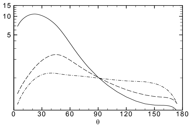
Figure 5.—As figure 4 but for a ring source at x_1^s/D_j = 7.5 and r^s/D_j : 0.0 (solid line); 0.50 (dashed line); 2.0 (dash-dot).
