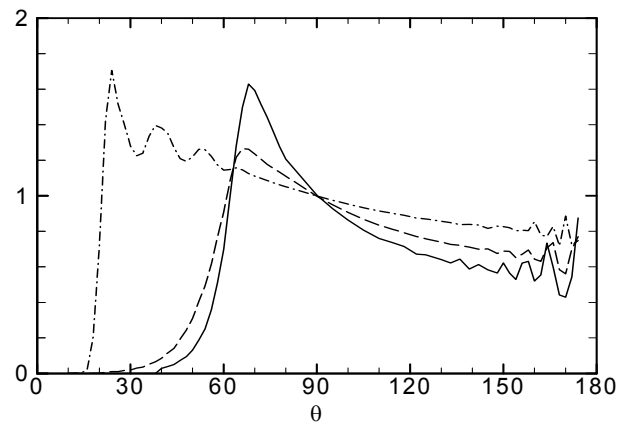
Figure 9(b).—As figure 8(a) but for a convecting ring source at observer St = 1.0 .
