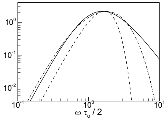
Figure 1.—Spectral shape function at 90^\circ with temporal function defined as: \exp(-|\tau/\tau_o|) , solid line; \exp\{-(0.4^2 + \tau^2/\tau_o^2)^{0.50}\} , dash-dot; \exp(-\tau^2/\tau_o^2) , dashed line.
