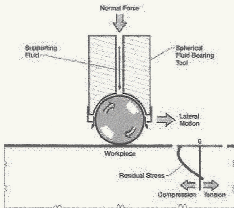
Figure 1 - LPB Schematic
