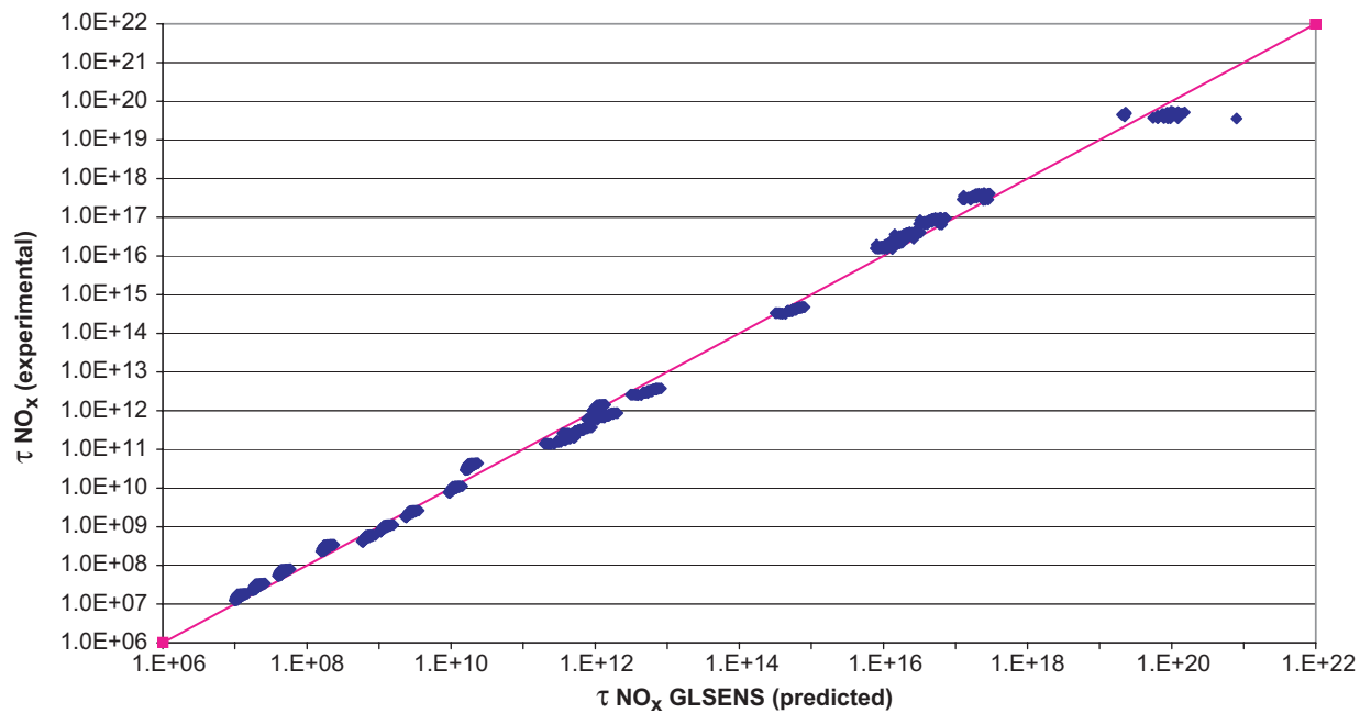
Figure 12. Kinetic methane \text{NO}_x \tau parity, step one (lean).
