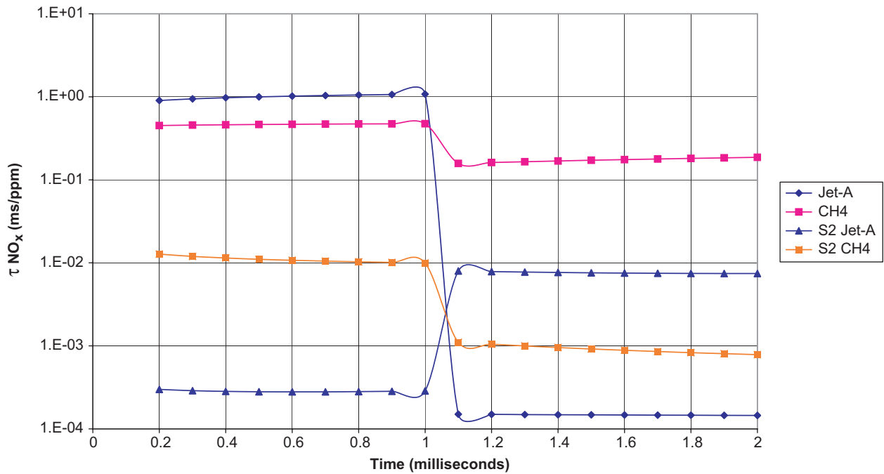
Figure 20a. Kinetic \tau_{NO_x} milliseconds/ppm at 10 atm and 2000 K for NO_x reaction step one and two (lean and rich) without water injection.
