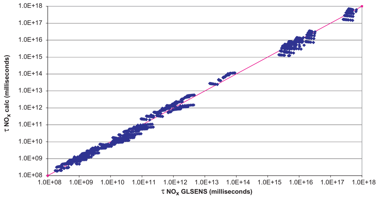
Figure 5. Kinetic Jet-A water injection NO x \tau parity, step one (lean).
