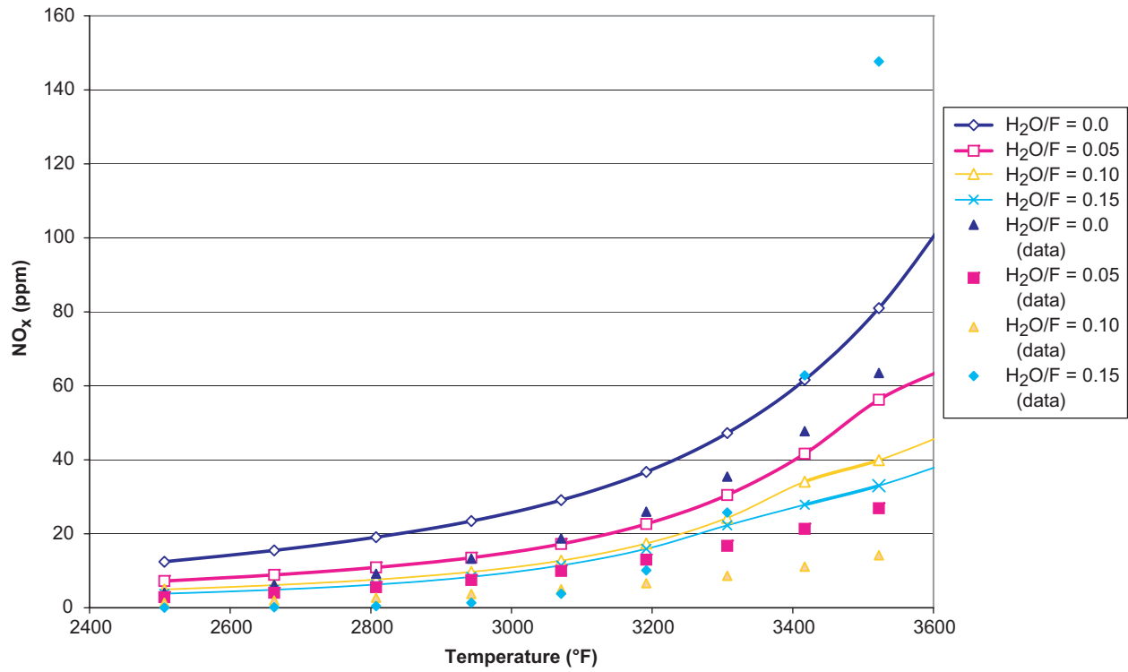
Figure 25. Methane NO x versus temperature.
