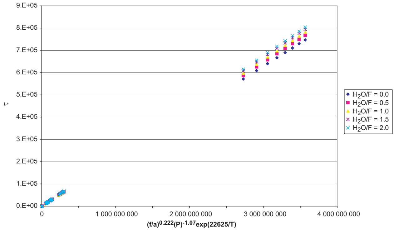
Figure 13. Methane fuel simple step one lean model.
