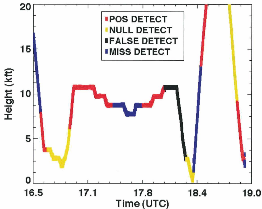
Figure 19. TAMDAR/Rosemont Comparison, December 11.
