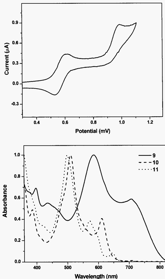
Fig. 4. (top) Cyclic voltammogram of CN-diox ( 9 ). The experiment was performed in benzonitrile (0.1 M TBAPF 6 ) at a scan rate of 50 mV/s. (bottom) Electronic spectra of the electrochemically generated radical cation of CN-diox ( 9 , solid line), Alkyl-diox ( 10 , dashed line), and diox ( 11 , dotted line) in benzonitrile.
