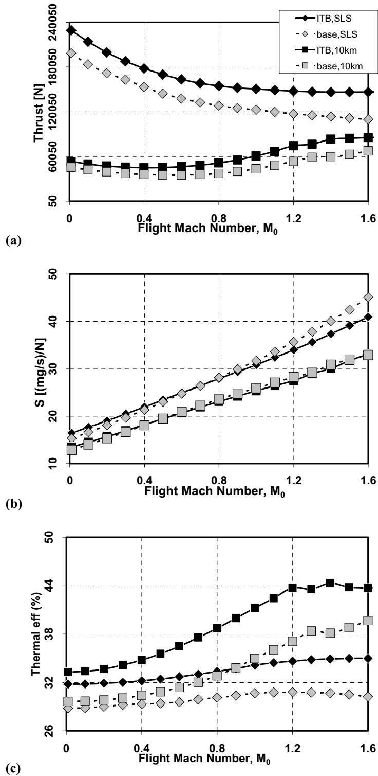
Figure 4. Full-throttle performance comparison of turbofan engines (case B) versus M_0 , \pi_{fR} = 2.2 , \pi_{cR} = 25 , T_{t4R} = 1550\text{K} , T_{t4.5R} = 1450\text{K} , \dot{m}_{0R} = 540\text{ kg/s} , and \alpha_R = 4.0 .
