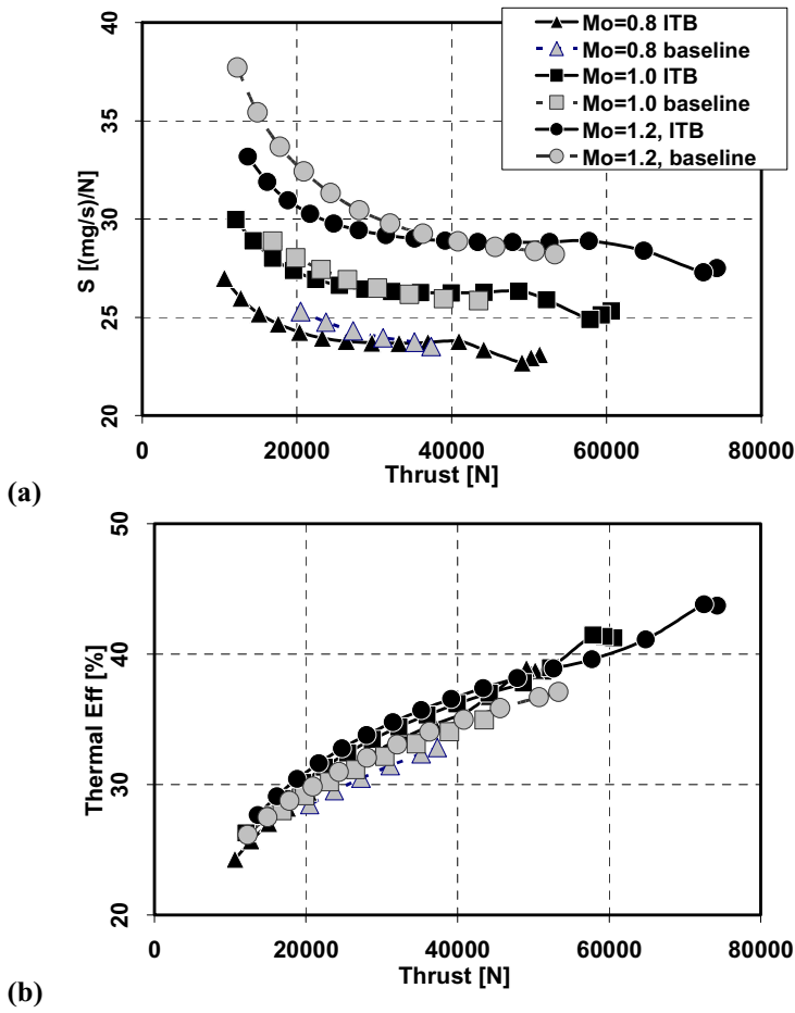
Figure 6. Partial-throttle performance of turbofan engine (case B) at altitude of 10km, \pi_{fR} = 2.2 , \pi_{cR} = 25 , T_{t4R} = 1550\text{K} , T_{t4.5R} = 1450\text{K} , \dot{m}_{oR} = 540 \text{ kg/s} , and \alpha_R = 4.0 .
