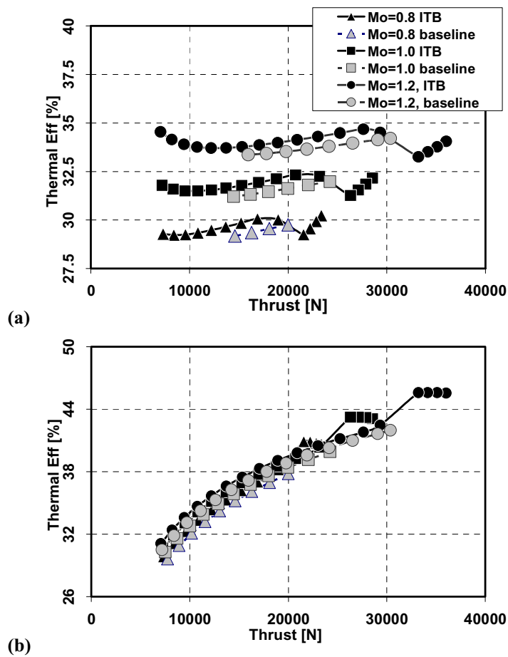
Figure 5. Partial-throttle performance of turbofan engine (case A) at altitude of 10km, \pi_{cR} = 2.43 , \pi_{cR} = 20 , T_{i4R} = 1450K , T_{i4.5R} = 1350K , \dot{m}_{0R} = 118 kg/s, and \alpha_R = 0.73 .
