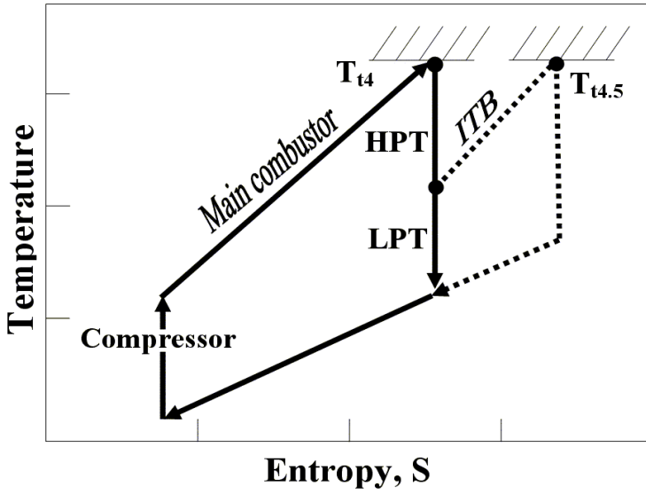
Figure 1. T-s diagram of a gas turbine engine with ITB
