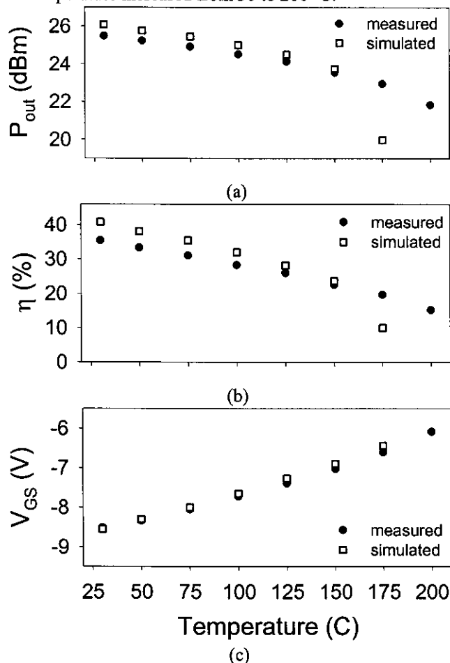
Fig. 7: Measured and simulated P_{out} (a), \eta (b), and V_{GS} (c) as a function of temperature.
