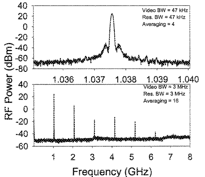
Fig. 6: Measured RF spectrum at 30 ^\circ\text{C} , I_{DS}=100 mA, V_{DS}=10 V.
