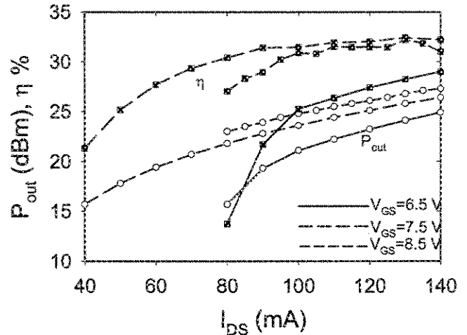
Fig. 5: Measured oscillator output power and efficiency, \eta , at 30 ^\circ\text{C} .
