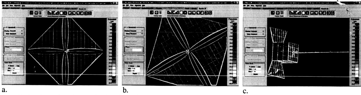
Figure 5. Surface charging analysis of candidate solar sail using Nascap-2k. Environment A (refer to Table 2) was used with sun incidence of 30^\circ from sail normal and a sun intensity of one (1). For this run, the backside of the solar sail is conductive (aluminum). Figures a, b, and c show a sun incident view (front), back view, and close up of the solar array spacecraft and connecting boom, respectively. Maximum charging levels can be seen in the eclipsed boom of -77.8 V. The sail front and back are 5.1 V, which yields a maximum differential charging from sail front to back of 0 V.
