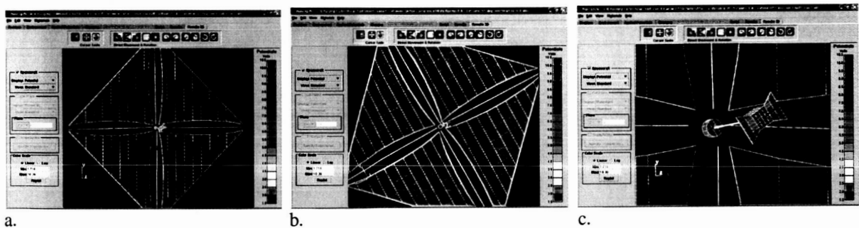
Figure 4. Surface charging analysis of candidate solar sail using Nascap-2k. Environment B (refer to Table 2) was used with sun incidence of 55^\circ from sail normal and a sun intensity of one (1). Figures a, b, and c show a sun incident view (front), back side view, and close up of the solar arrays, respectively. All charging levels are positive for this run, with a maximum differential charging from sail front to back of 6.4 V.
