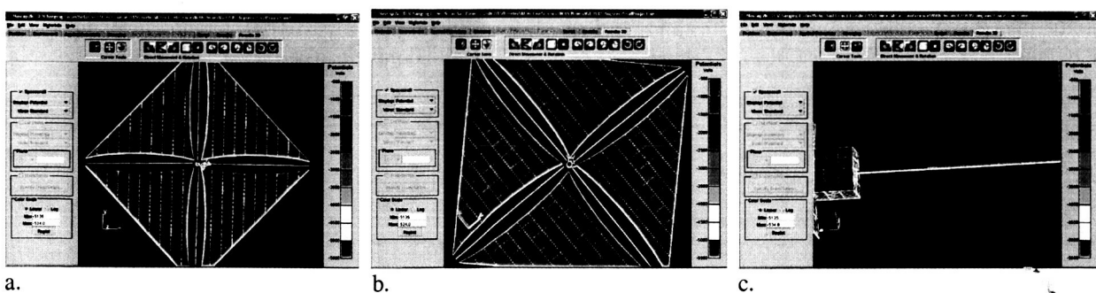
Figure 6. Surface charging analysis of candidate solar sail using Nascap-2k. Geosynchronous environment (refer to Table 2) was used with a sun incidence 30° from normal to the sail front and a sun intensity of one (1). Figures a, b, and c show a sun incident view (front), back side view, and close up of the solar array spacecraft and connecting boom, respectively. Maximum charging levels can be seen in the eclipse side of the boom of -5135 V. Maximum differential charging levels from the sail front to sail back are 230 V.
